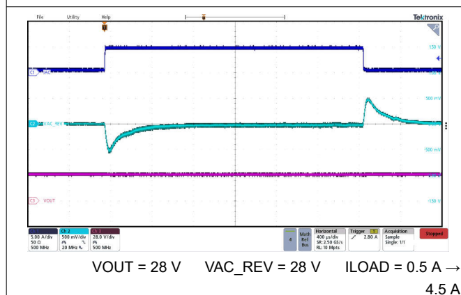
Figure 7-23. Reverse Mode Buck-Boost Transient Reponse
