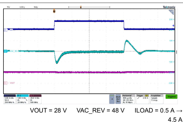
Figure 7-24. Reverse Mode Boost Transient Reponse
