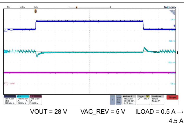
Figure 7-22. Reverse Mode Buck Transient Reponse
