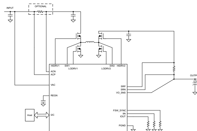
Simplified Schematic
