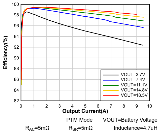
Figure 8-5. PTM Mode Charge Efficiency
