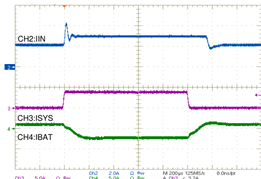
Figure 9-16. Input Current in Boost Mode
