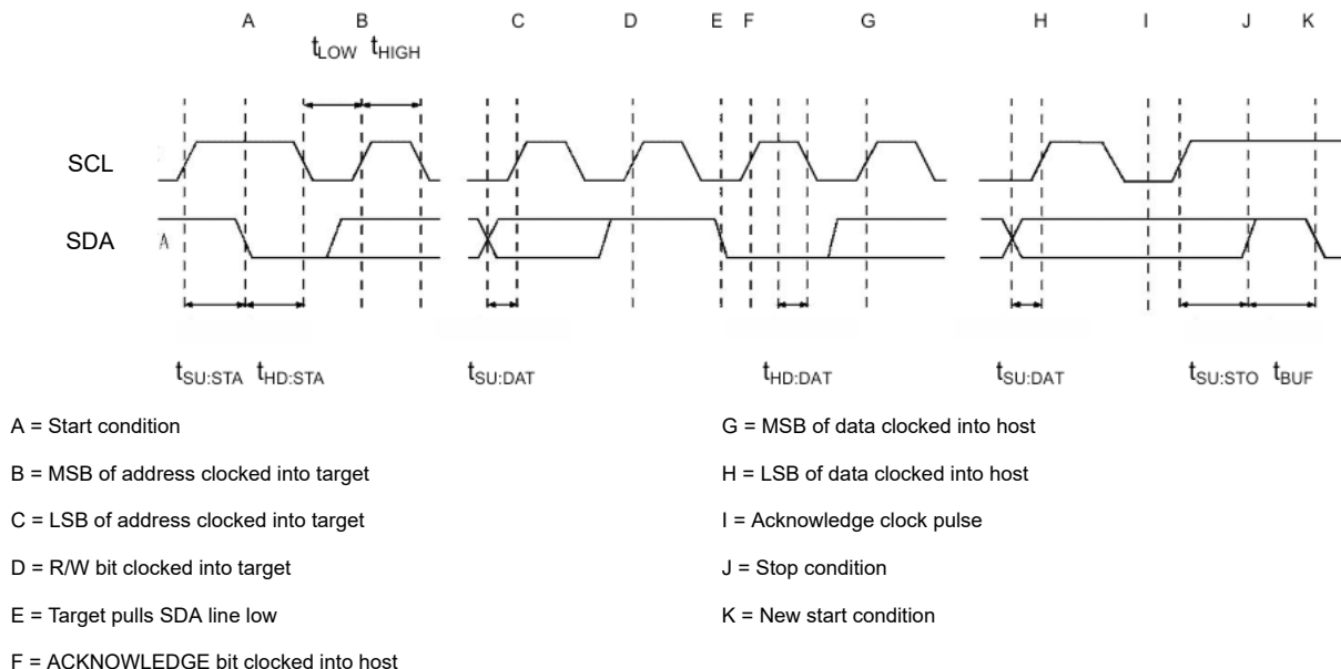
Figure 8-7. I²C Read Timing
