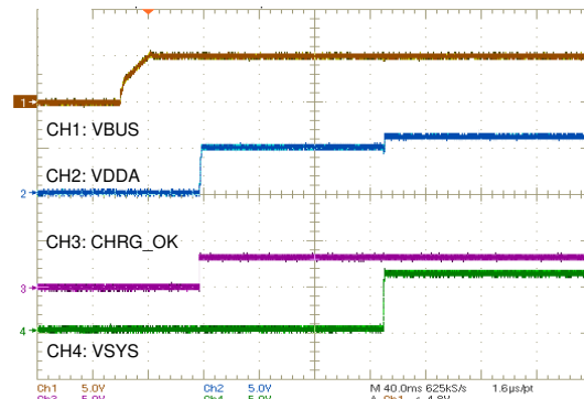
Figure 9-5. Power Up From 5 V
