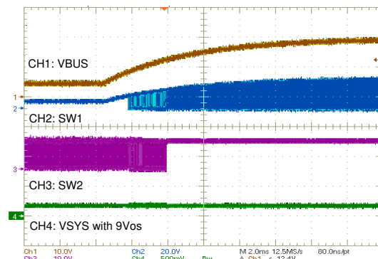
Figure 9-5. Power Up From 5 V
