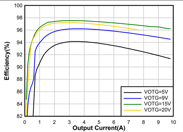
Figure 7-13. OTG Efficiency with 4S Battery
