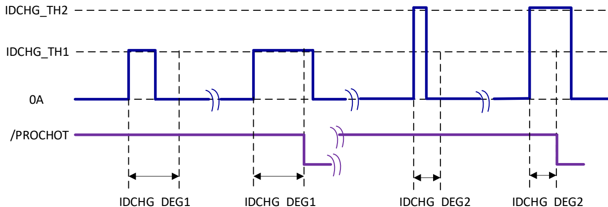
Figure 8-1. Two-Level Battery Discharging Current Trigger \overline{\text{PROCHOT}} Diagram
