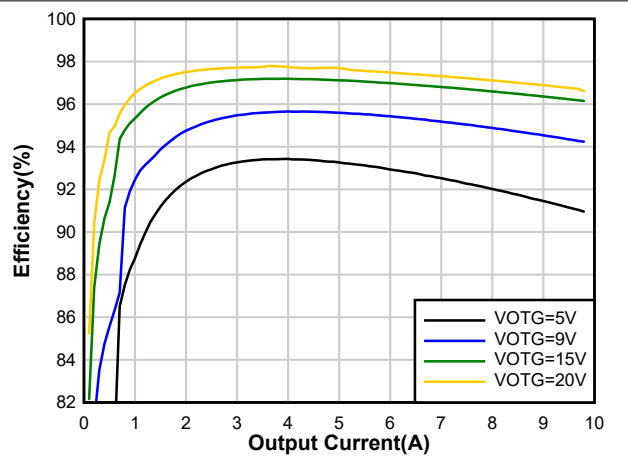
Figure 7-14. OTG Efficiency with 5S Battery
