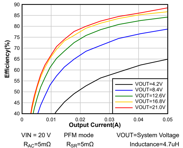
Figure 7-4. Light Load System Efficiency
