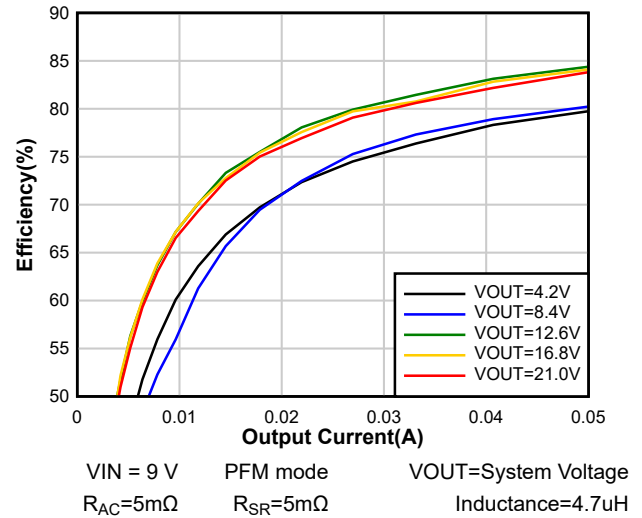
Figure 7-2. Light Load System Efficiency
