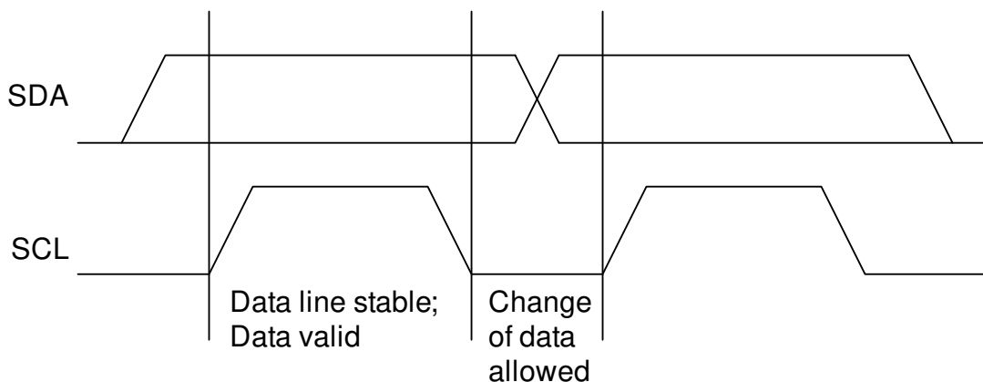
Figure 8-8. Bit Transfer on the I²C Bus
