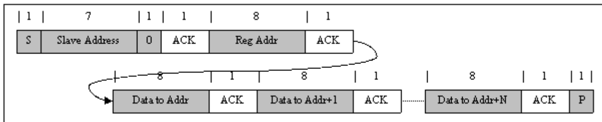
Figure 8-14. Multi Write
