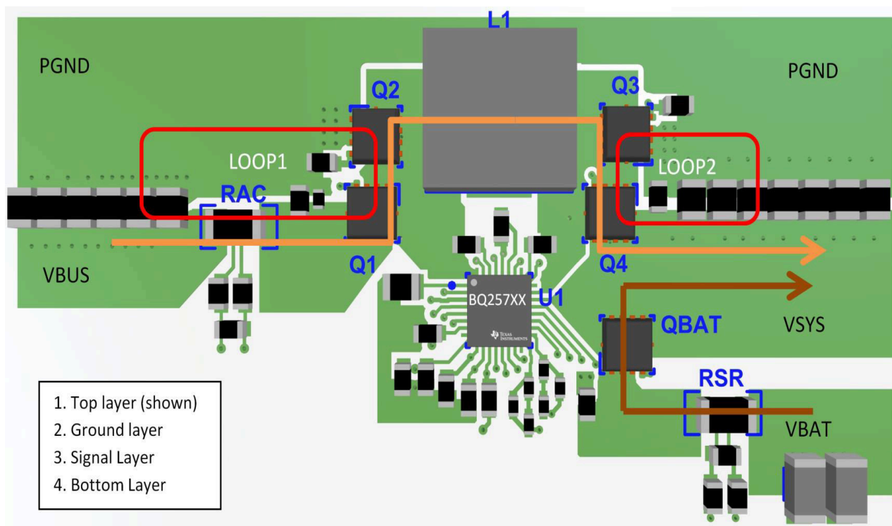
Figure 11-1. Buck-Boost Charger Layout Reference Example Top View
