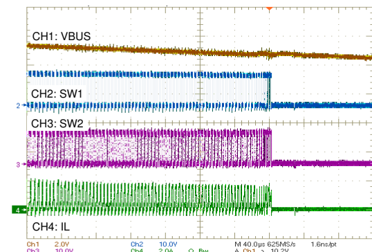
Figure 9-4. Power Up From 20 V
