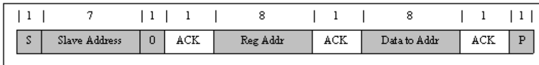
Figure 8-12. Single Write
