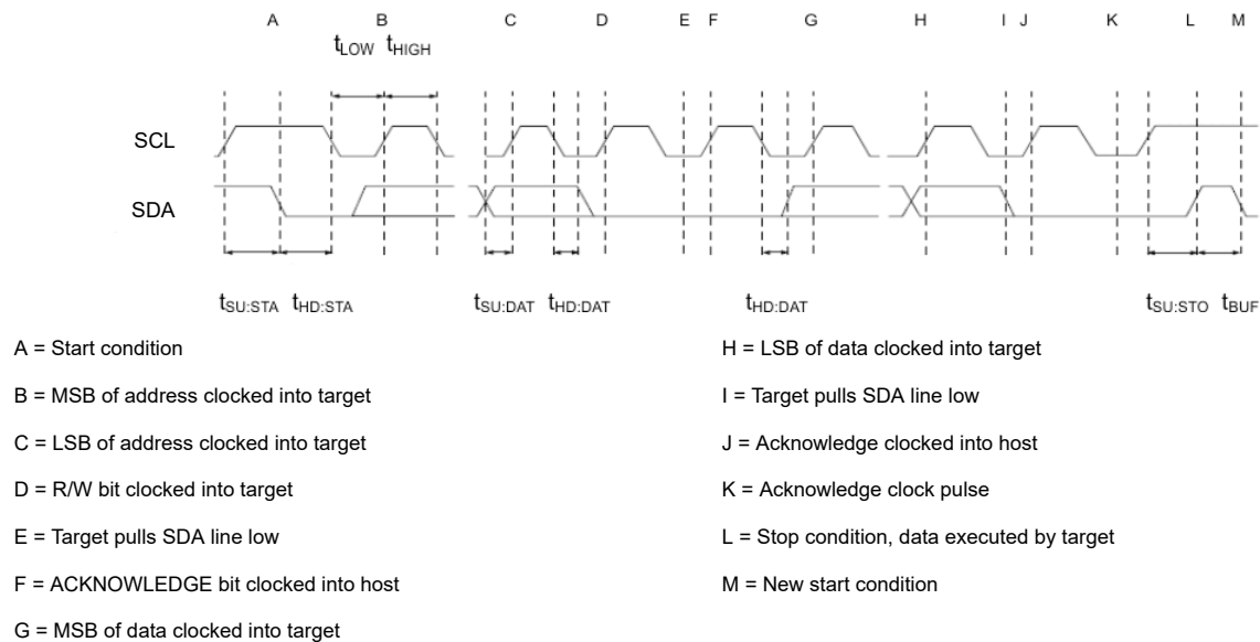
Figure 8-6. I 2 C Write Timing
