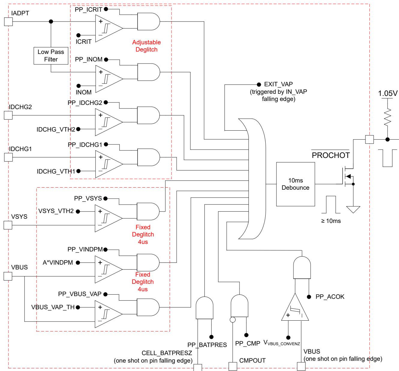
Figure 8-4. \overline{\text{PROCHOT}} Profile
