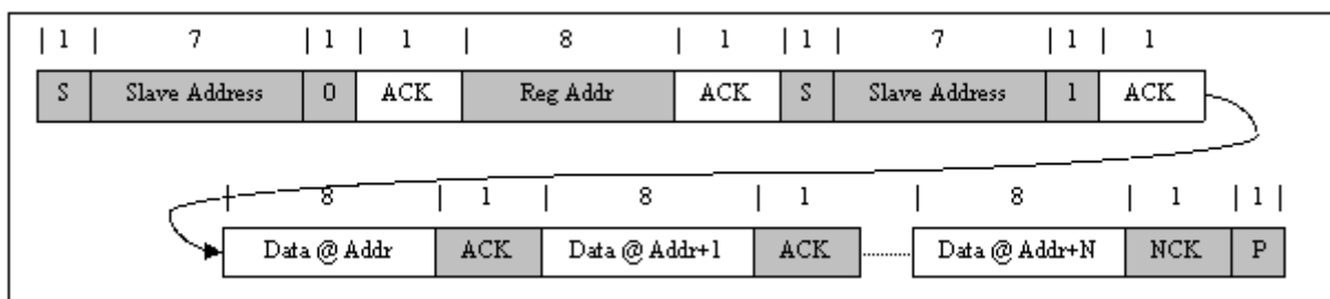
Figure 8-15. Multi Read
