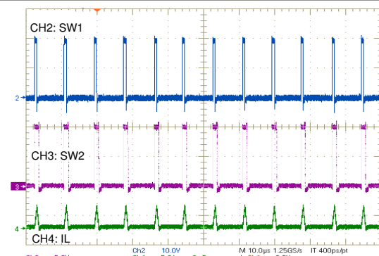
Figure 9-6. Power Off From 12 V
