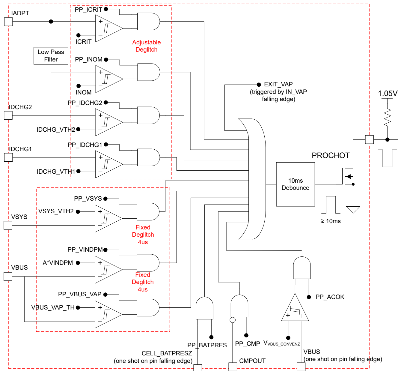
Figure 9-4. \overline{\text{PROCHOT}} Profile
