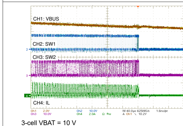
Figure 10-5. Power Off from 12 V
