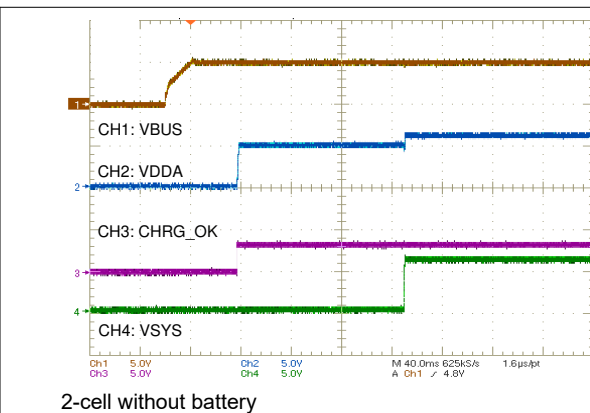
Figure 10-4. Power Up from 5 V
