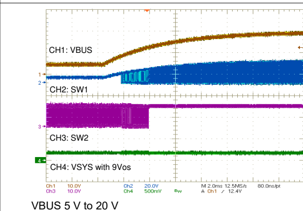
Figure 10-6. System Regulation
