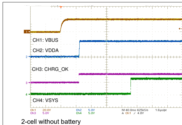
Figure 10-3. Power Up from 20 V
