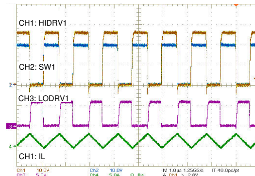
Figure 10-8. PWM Operation
