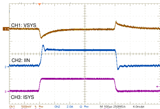
Figure 10-9. Switching During Boost Mode
