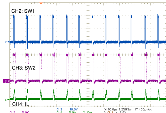
Figure 10-7. PFM Operation
