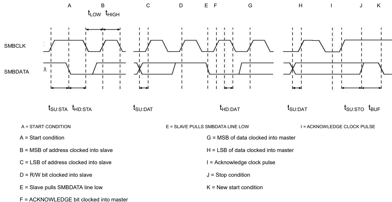
Figure 9-5. SMBus Read Timing
