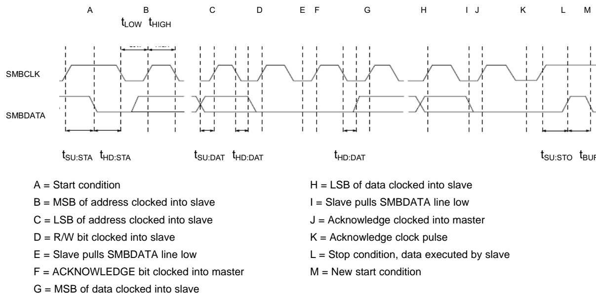
Figure 15. SMBus Write Timing
