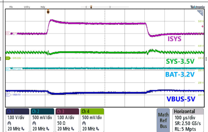
Figure 8-5. Charge Enable
