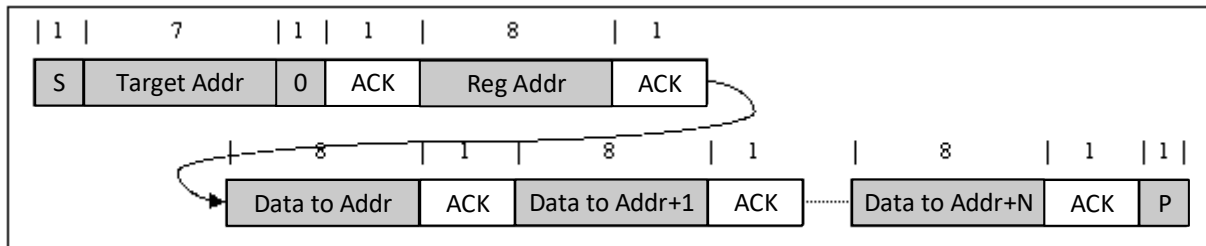
Figure 7-15. Multi-Write
