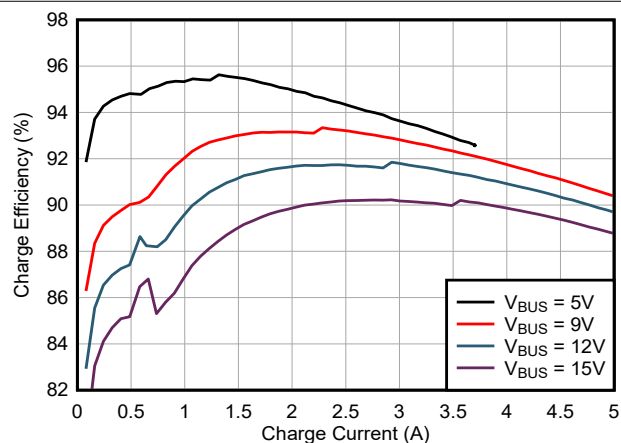
Figure 6-1. Charge Efficiency vs Charge Current
