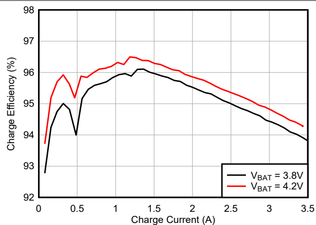
Figure 6-2. Charge Efficiency vs Charge Current
