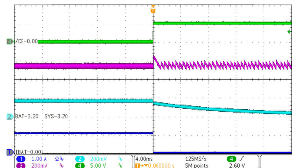
Figure 9-3. Power-Down
