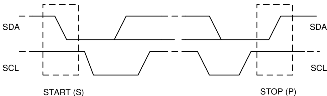
Figure 8-8. START and STOP Conditions on the I²C Bus
