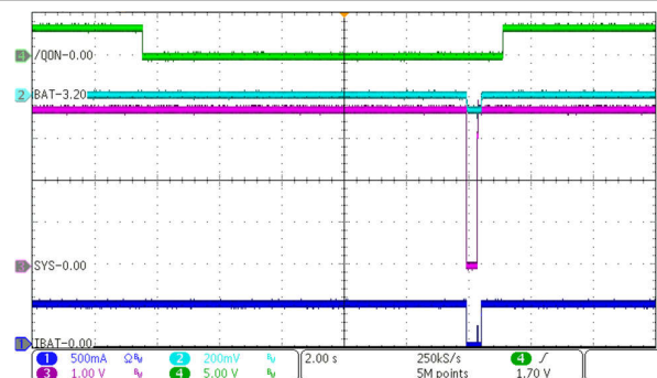
Figure 9-5. Charge Disable
