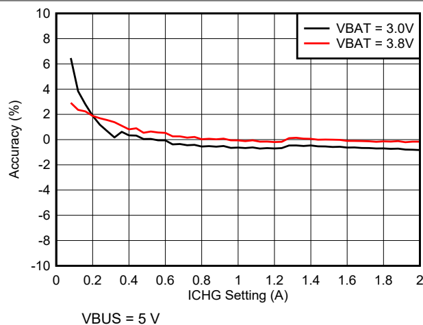
Figure 7-3. Charge Current Accuracy vs ICHG Setting
