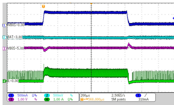
Figure 9-16. Boost Mode Load Transient
