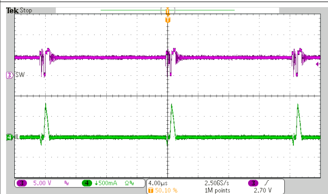
Figure 10-9. Charge Enable
