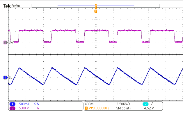
Figure 10-11. OTG Switching
