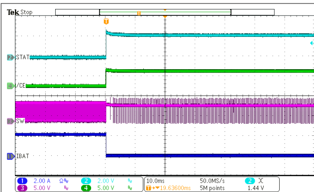
Figure 9-11. Charge Disable
