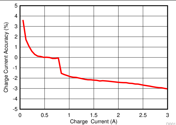
Figure 7-4. Charge Current Accuracy
