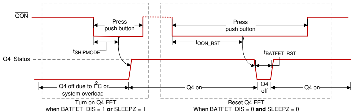
Figure 8-10. \overline{QON} Timing
