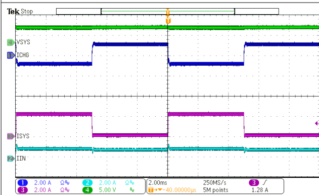
Figure 9-13. OTG Switching
