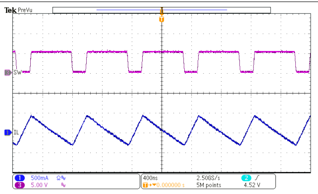
Figure 9-12. OTG Switching
