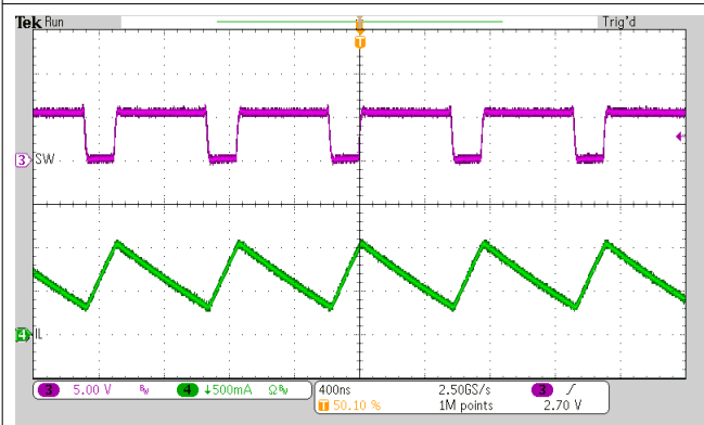
Figure 9-11. Charge Disable
