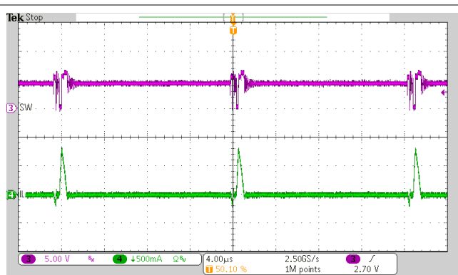
Figure 9-12. OTG Switching
