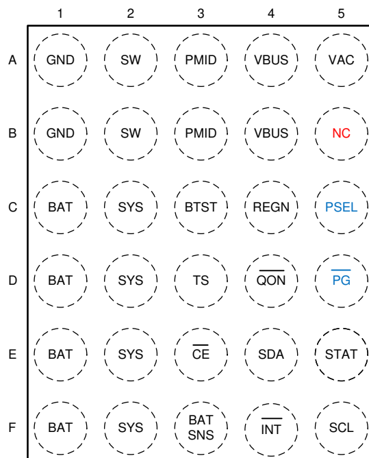
Figure 6-1. BQ25600 YFF Package 30-Pin WCSP Top View
