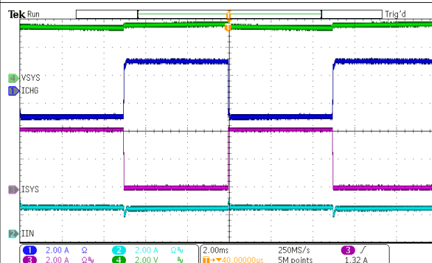
Figure 9-18. System Load Transient
