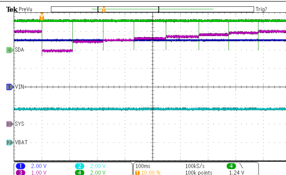
Figure 8-13. SYS Regulation Sweep
