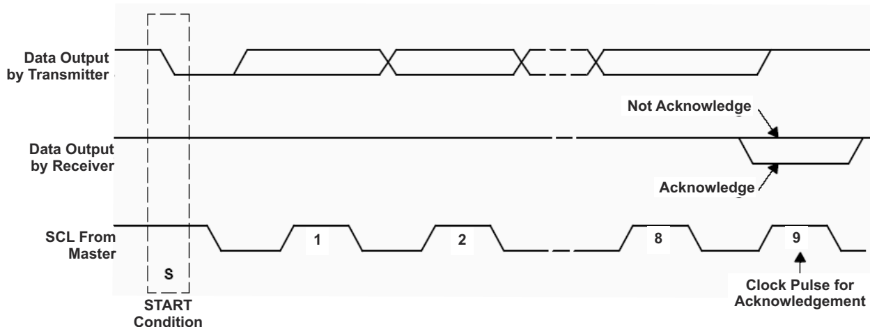
Figure 8-8. Acknowledge on the I 2 C Bus
