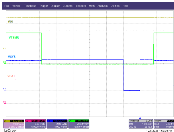
Figure 9-6. Hardware Reset with /TSMR Press
