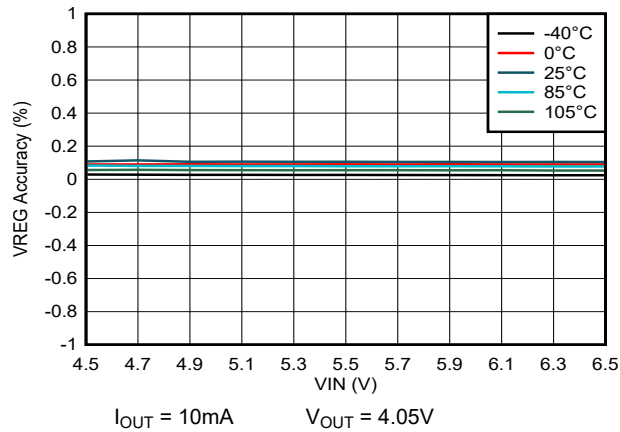
Figure 5-1. Line Regulation
