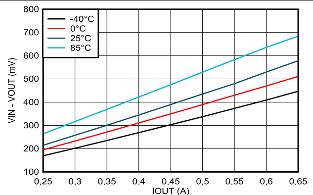
Figure 5-6. Dropout Voltage vs Output Current
