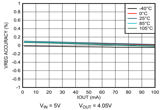
Figure 5-2. Load Regulation
