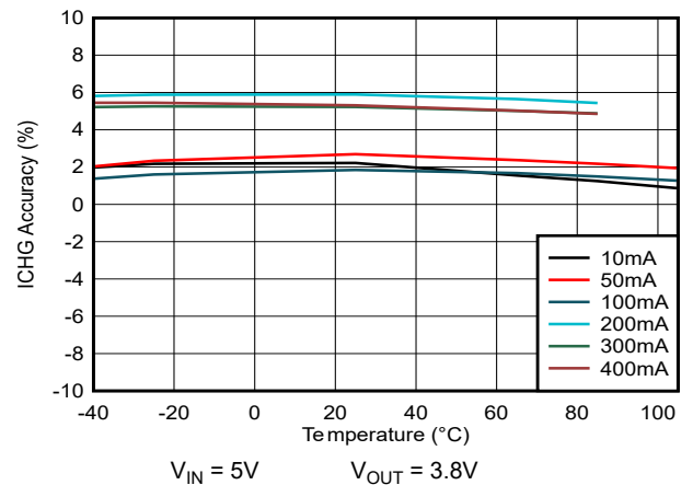
Figure 5-4. ICHG Accuracy vs Temperature
