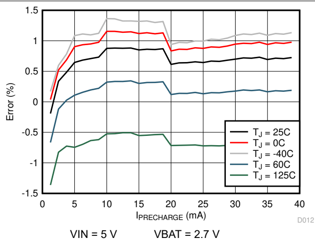
Figure 8-3. Pre-Charge Current Accuracy vs. IPRECHARGE Setting (ICHARGE_RANGE = 0)
