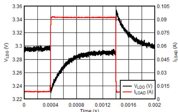
Figure 10-19. LDO Load Transient - VLDO = 3.3 V
