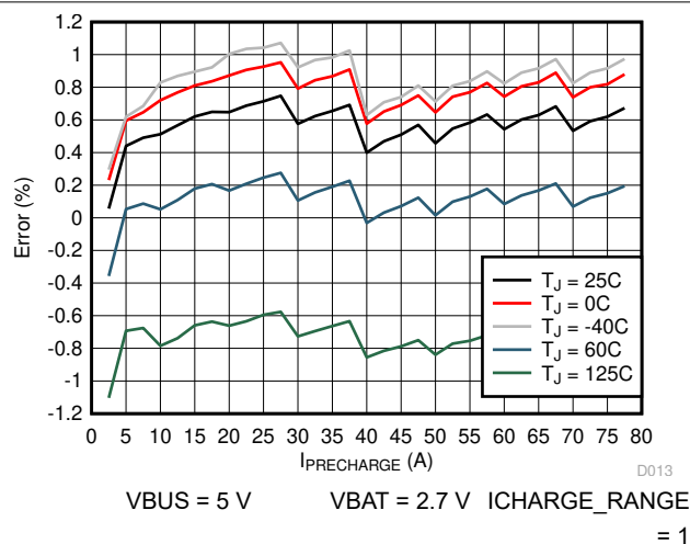
Figure 8-4. Pre-Charge Current Accuracy vs. IPRECHARGE Setting (ICHARGE_RANGE = 1)
