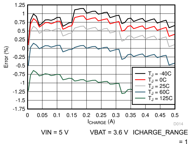
Figure 8-2. Charge Current Accuracy vs. ICHARGE Setting
