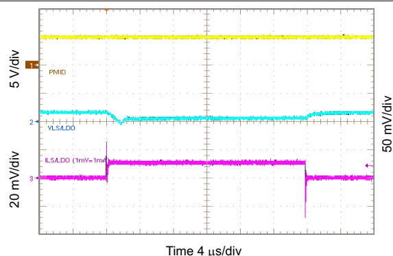
Figure 10-48. 2.5 V LSLDO Load Transient, 0 to 10 mA
