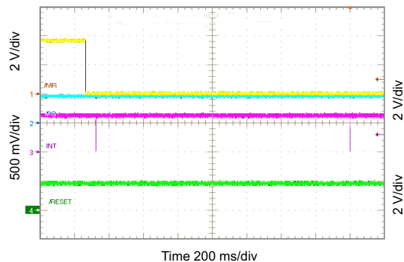
Figure 10-60. \overline{\text{PG}} Functions as Shifted \overline{\text{MR}} Output
