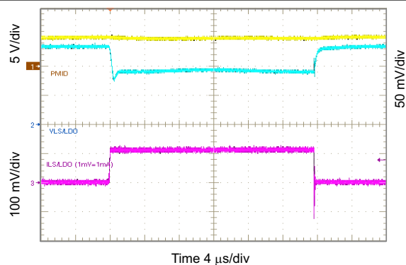
Figure 10-54. 3.3 V L SLDO Load Transient, 0 to 100 mA
