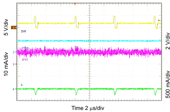
Figure 10-27. Light Load Operation Showing SW
