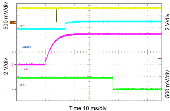
Figure 10-57. Show \overline{\text{PG}} and \overline{\text{INT}} Timing ( \text{V}_{\text{IN}} Insertion)
