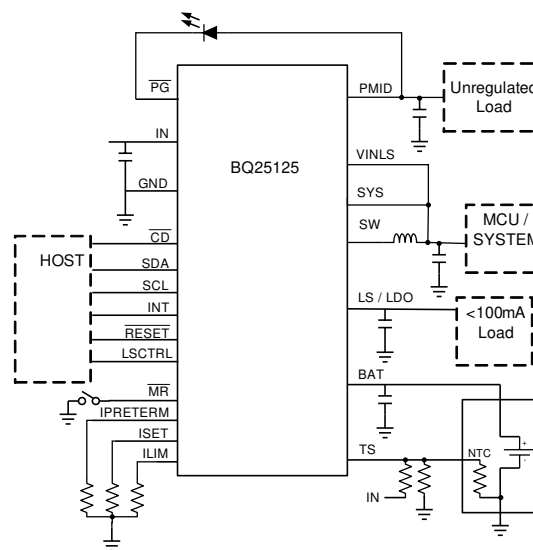
Simplified Schematic
