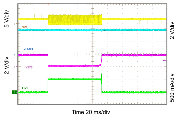
Figure 10-42. Short Circuit and Recovery for SYS
