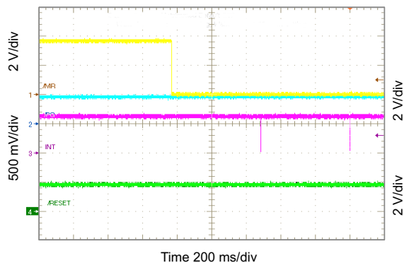
Figure 10-59. \overline{\text{PG}} Functions as Shifted \overline{\text{MR}} Output
