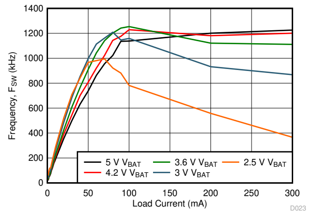
Figure 10-23. 1.8 V_{\text{SYS}} Switching Frequency vs Load Current
