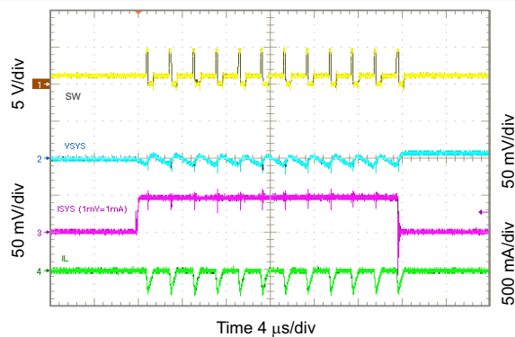
Figure 10-31. 1.2 V_{SYS} Load Transient, 0 to 50 mA
