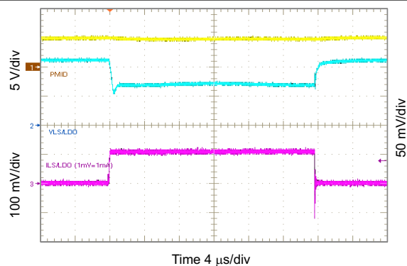
Figure 10-53. 2.5 V L SLDO Load Transient, 0 to 100 mA
