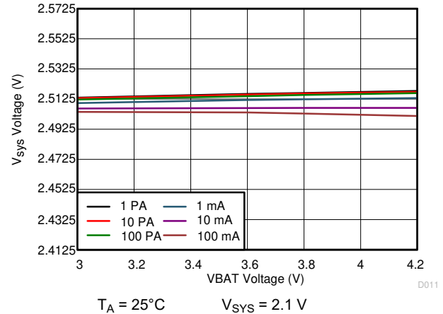
Figure 10-21. 2.1 V_{\text{SYS}} Line Regulation
