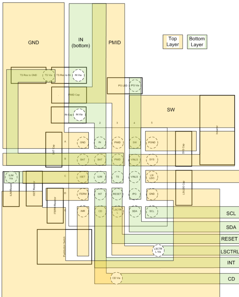
Figure 12-1. BQ25122 Layout
