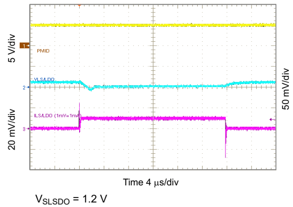
Figure 10-48. 1.2 V LSLDO Load Transient, 0 to 10 mA
