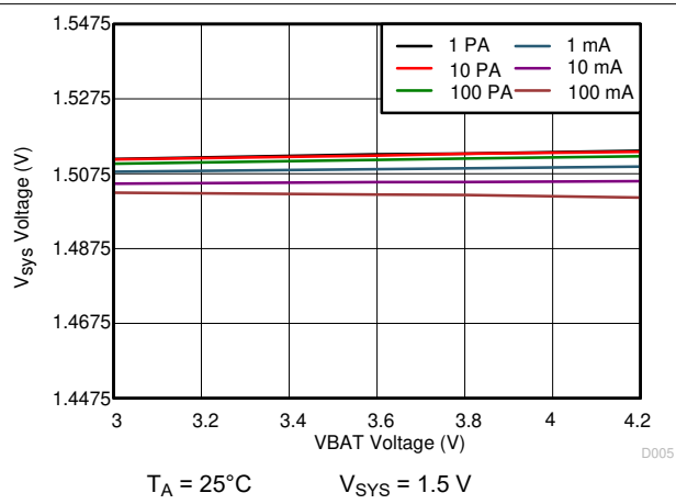
Figure 10-21. 1.5 V sys Line Regulation
