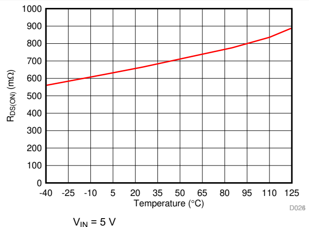
Figure 8-12. R_{DS(ON)} of High Side MOSFET vs Temperature
