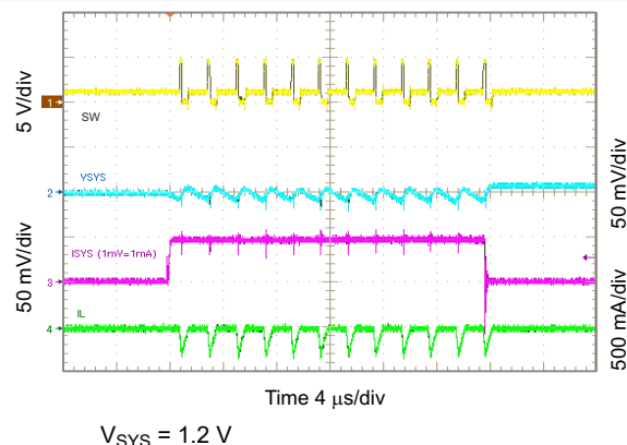
Figure 10-33. 1.2 V SYS Load Transient, 0 to 50 mA
