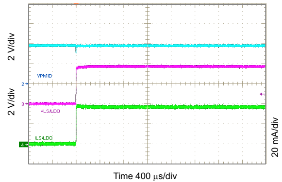
Figure 10-46. Startup Showing SS on LS/LDO Output
