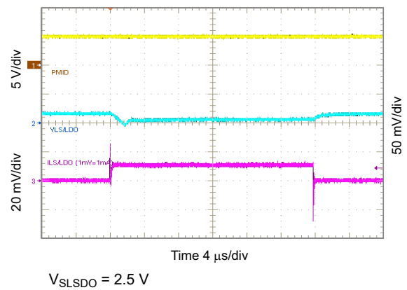
Figure 10-50. 2.5 V LSLDO Load Transient, 0 to 10 mA
