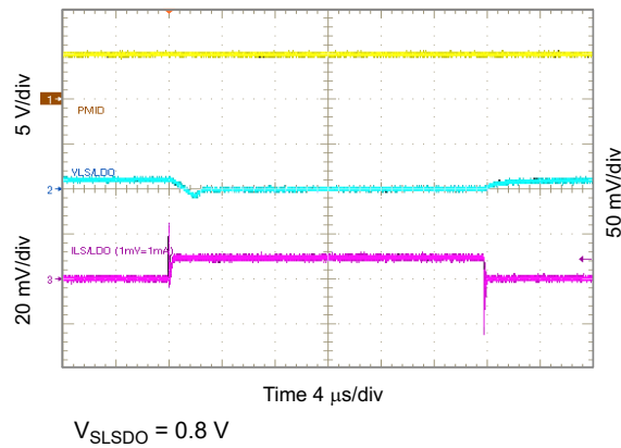
Figure 10-47. 0.8 V LSLDO Load Transient, 0 to 10 mA
