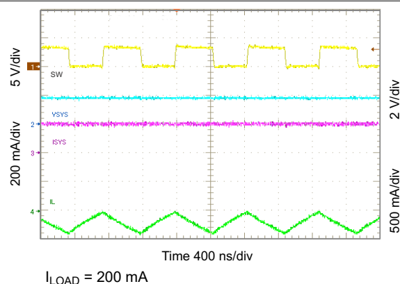
Figure 10-31. Light Load Operation Showing SW
