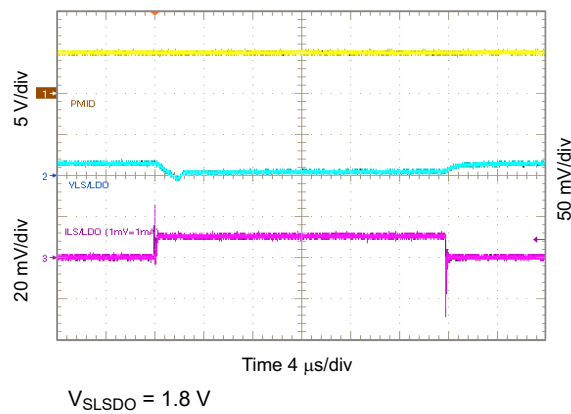
Figure 10-49. 1.8 V LSLDO Load Transient, 0 to 10 mA
