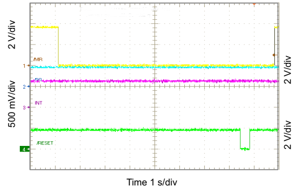
Figure 10-66. RESET Timing
