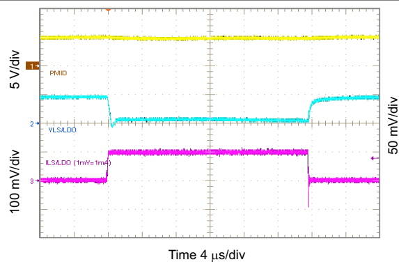
Figure 10-52. 0.8 V LSDO Load Transient, 0 to 100 mA
