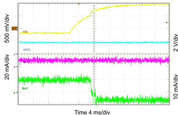
Figure 10-9. OVP Fault
