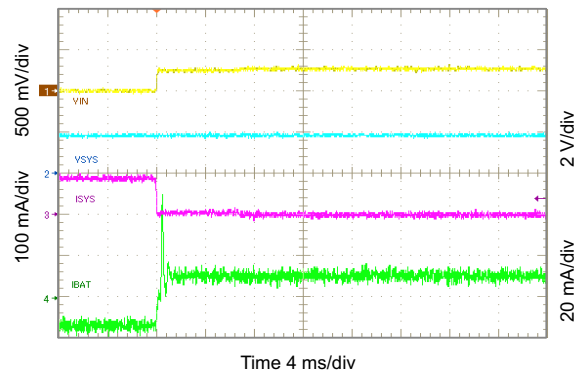
Figure 10-7. Exiting Battery Supplement Mode
