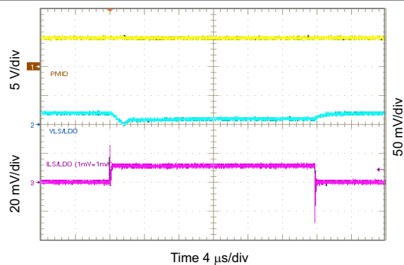
Figure 10-51. 3.3 V LSDO Load Transient, 0 to 10 mA
