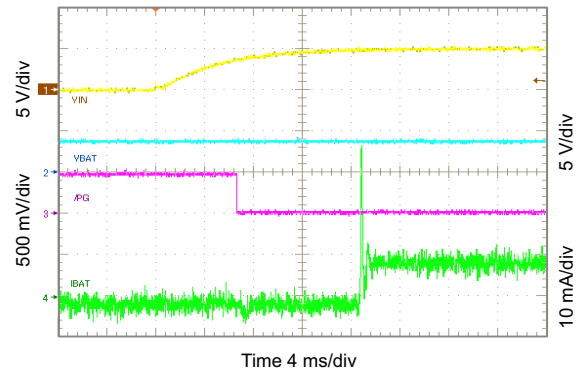
Figure 10-3. Power Supply Connected to V_{IN}
