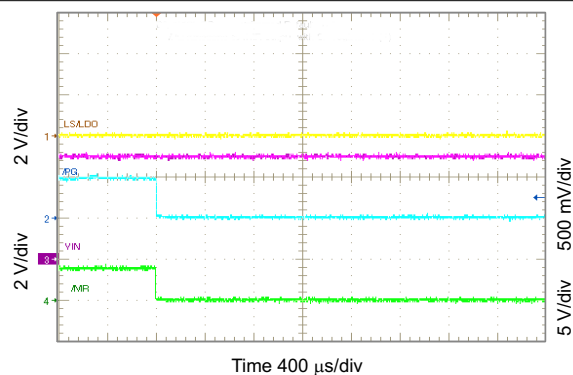
Figure 10-61. \overline{\text{PG}} Functions as Shifted \overline{\text{MR}} Output
