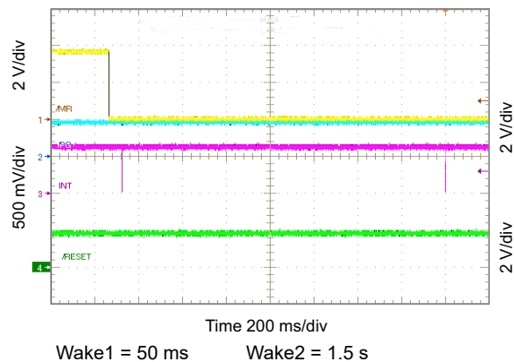
Figure 10-64. Show \overline{\text{MR}} Timing
