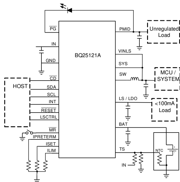
Simplified Schematic
