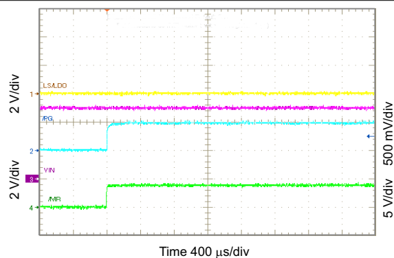
Figure 10-62. \overline{\text{PG}} Functions as Shifted \overline{\text{MR}} Output
