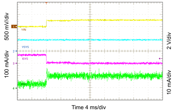
Figure 10-5. Exiting DPPM Mode
