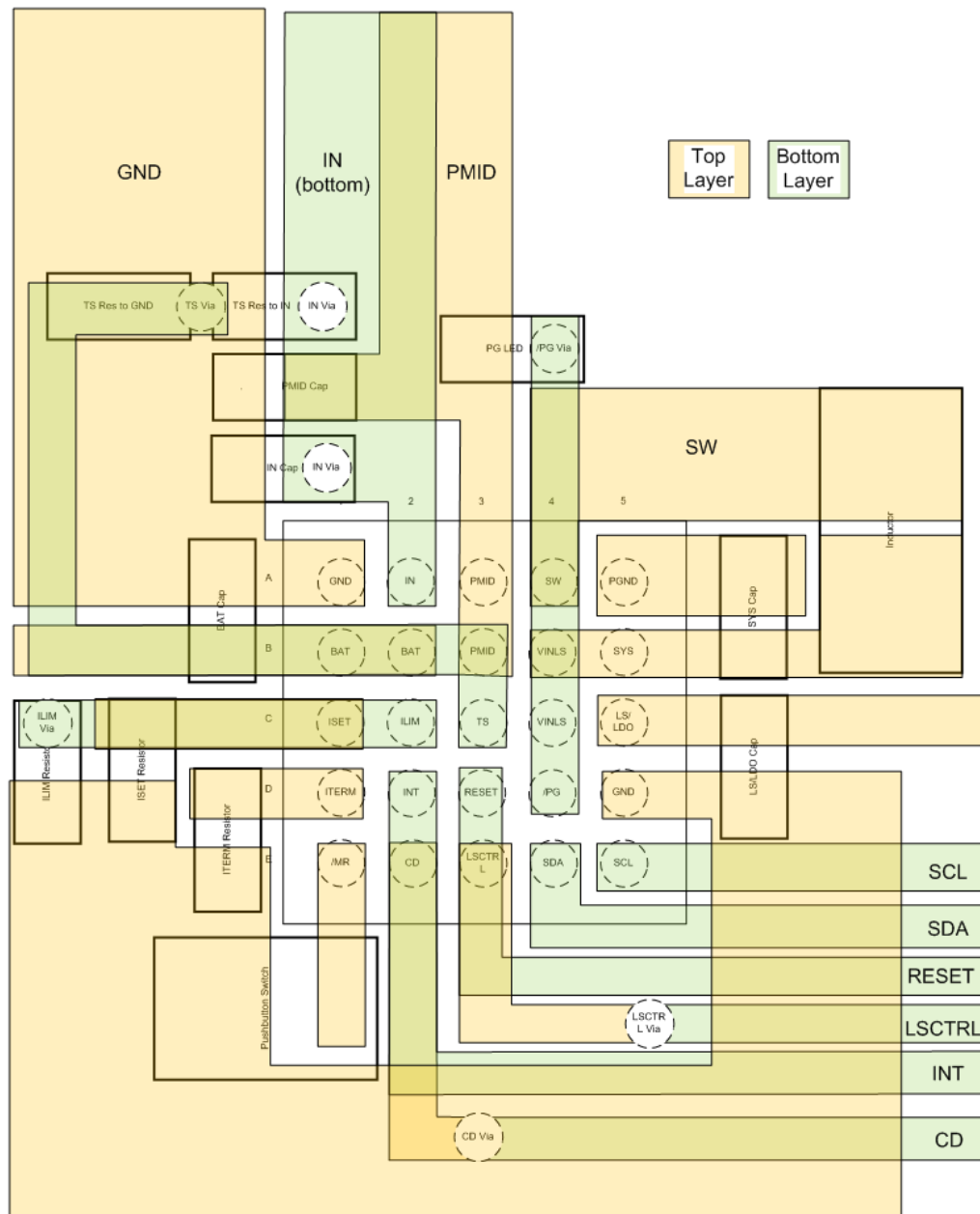
Figure 12-1. BQ25121A Layout
