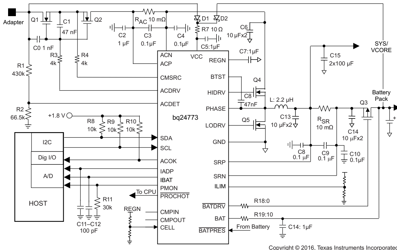
Figure 36. bq24773 Typical Schematic
