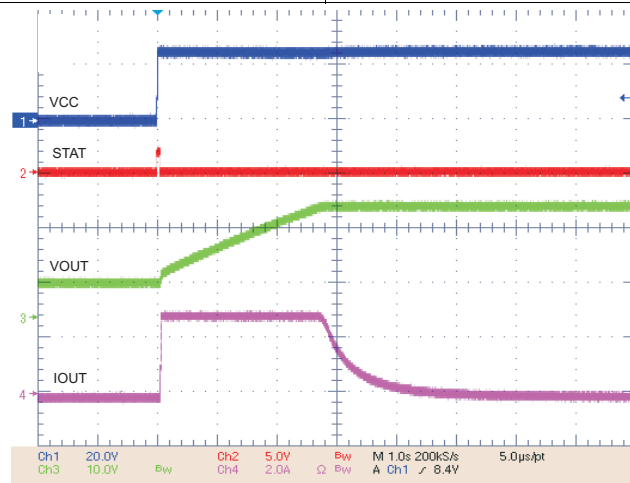
Figure 5. Continuous Conduction Mode
