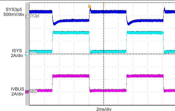
Figure 42. PWM Switching in Buck Mode
