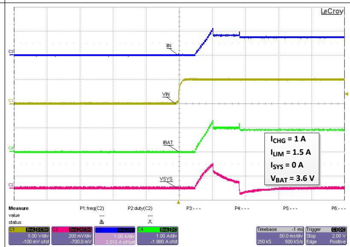
Figure 10. Startup
