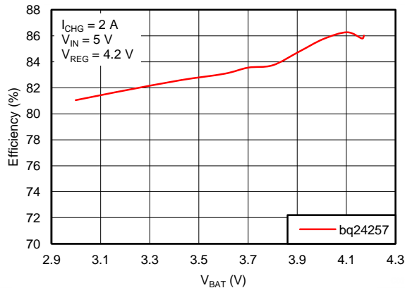
Figure 3. Efficiency vs. Battery Voltage
