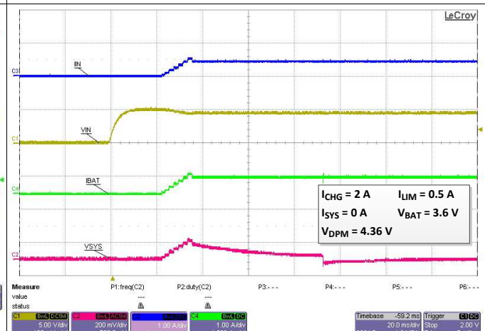
Figure 12. V_{DPM} Startup, 4.2 V
