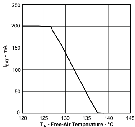
Figure 1. Thermal Regulation
