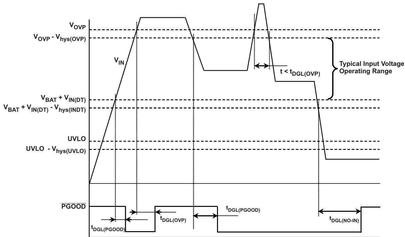
Figure 16. Power Up, Power Down
