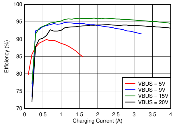
Figure 7-2. 3s Battery Charge Efficiency vs. Charge Current
