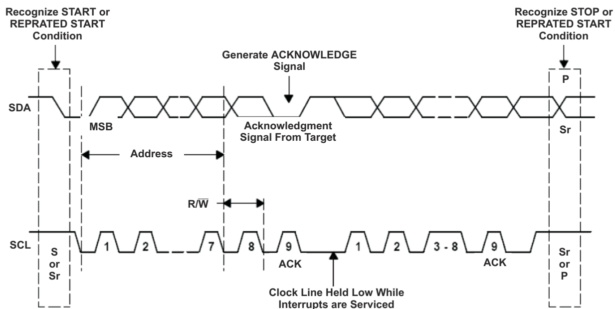
Figure 8-11. Bus Protocol
