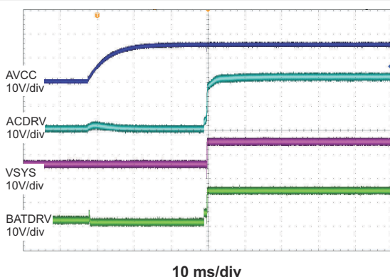
Figure 8-7. BATFET to ACFET Transition During Power Up
