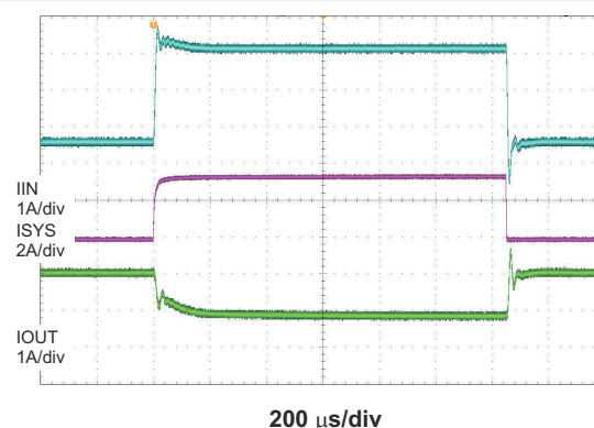
Figure 8-8. System Load Transient (Input current DPM)
