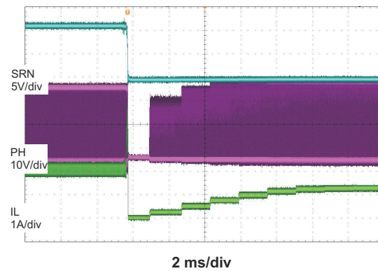
Figure 8-10. Battery to Ground Short Protection
