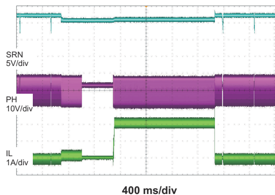
Figure 8-9. Battery Insertion and Removal
