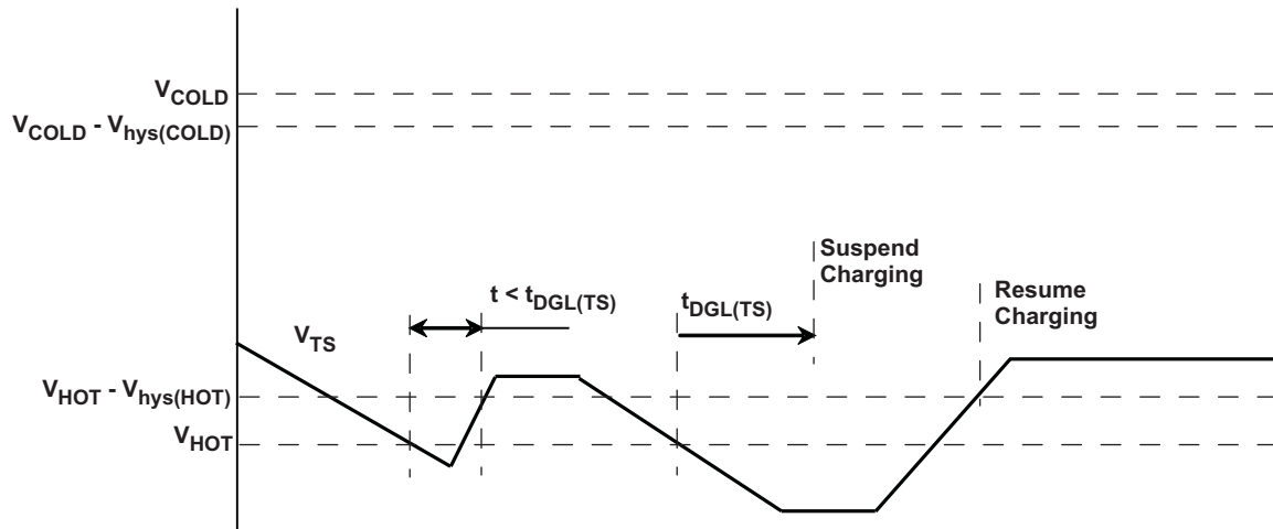
Figure 5. Battery Pack Temperature Sensing – TS Pin. Battery Temperature Increasing
