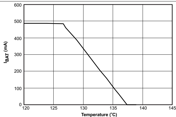
Figure 6. Thermal Regulation
