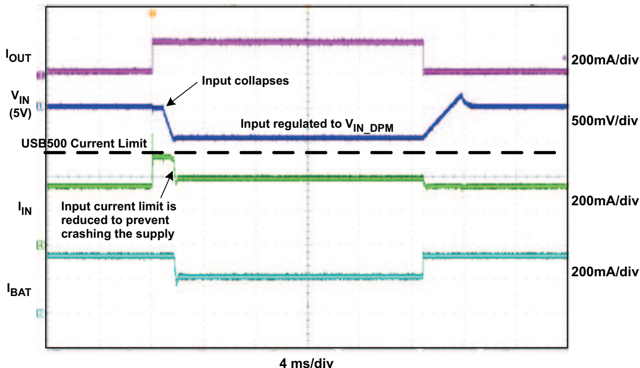
Figure 21. V_{IN\_DPM} Waveform
