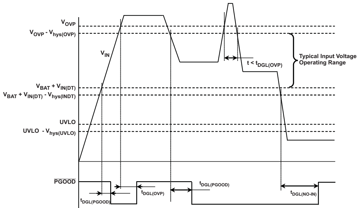
Figure 1. Power-Up, Power-Down, Power Good Indication
