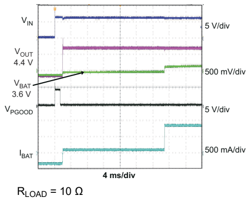
Figure 10-2. Adapter Plug-In Battery Connected
