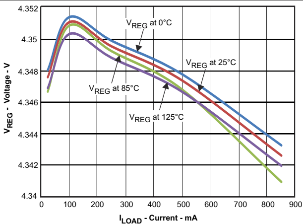
Figure 7-4. Load Regulation
