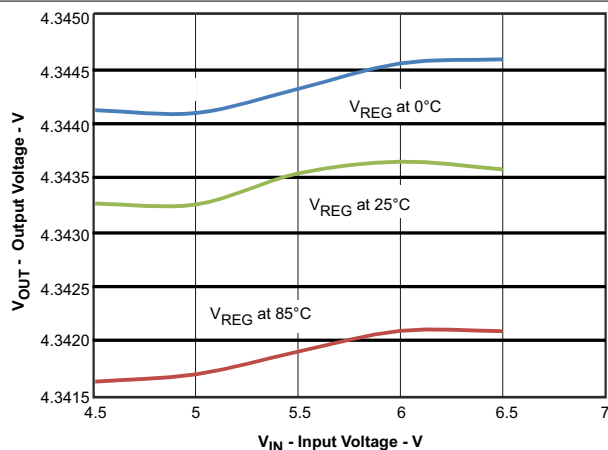
Figure 7-5. Line Regulation
