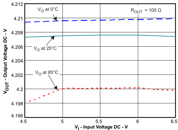
Figure 7-2. Line Regulation
