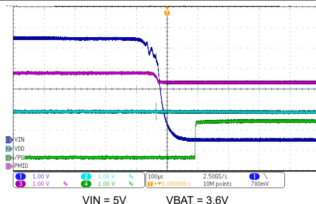
Figure 8-11. \overline{\text{PG}} Power Good Function - IN Supply Removal
