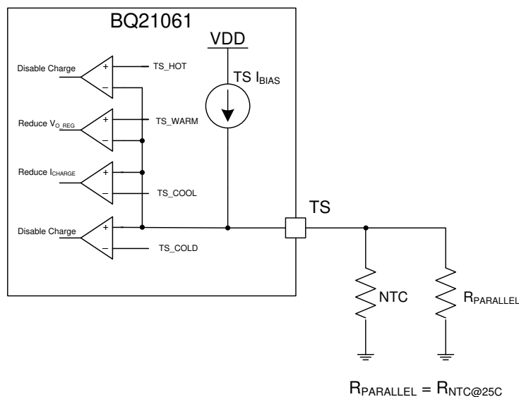
Figure 7-8. TS Bias Functional Diagram
