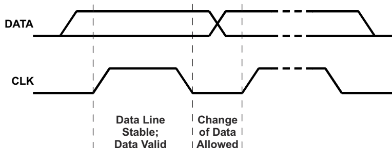
Figure 7-10. Bit Transfer on the Serial Interface
