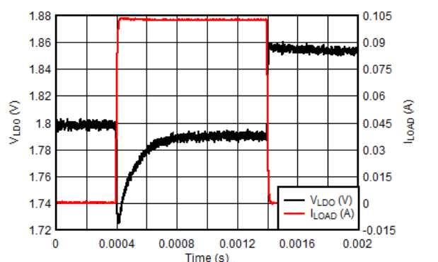
Figure 8-18. LDO Load Transient - VLDO = 1.8V
