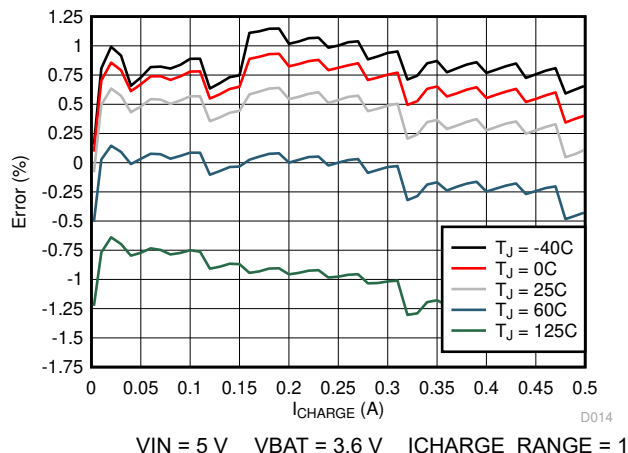
Figure 6-2. Charge Current Accuracy vs. ICHARGE Setting
