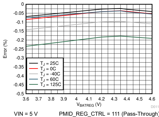
Figure 6-1. Battery Regulation Voltage Accuracy vs. VBATREG Setting
