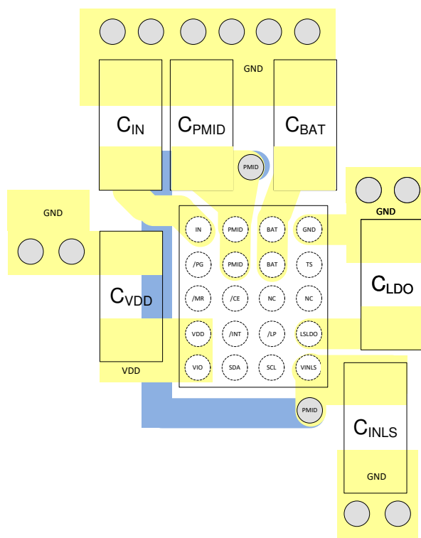
Figure 10-1. Layout Example
