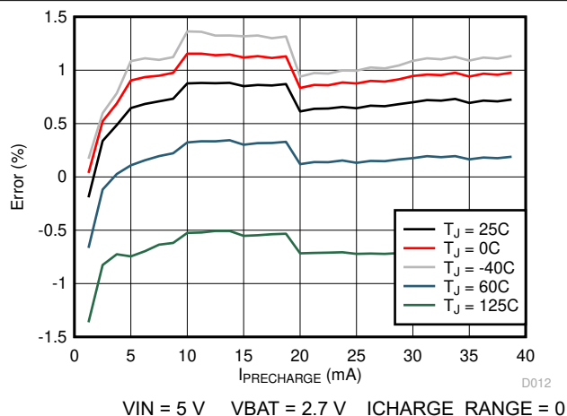
Figure 6-3. Pre-Charge Current Accuracy vs. IPRECHARGE setting (ICHARGE_RANGE = 0)
