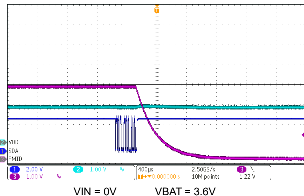
Figure 8-8. HW Reset Through I 2 C Command
