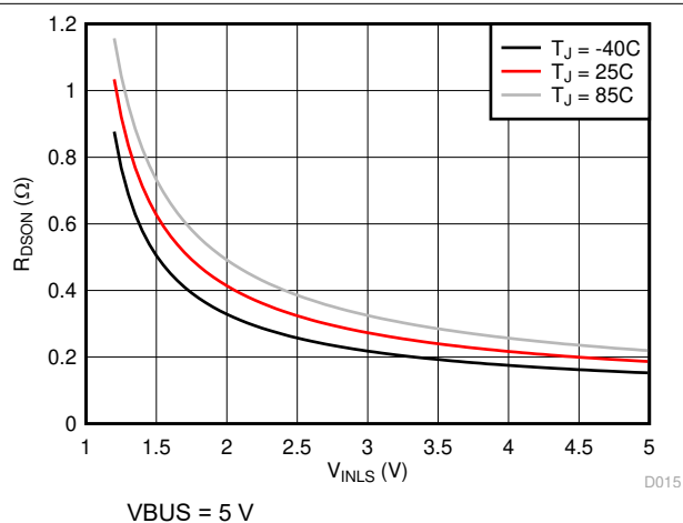
Figure 6-5. LS/LDO Switch On Resistance vs. VINLS
