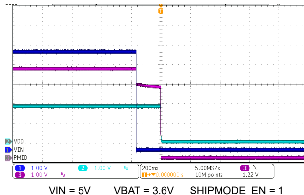
Figure 8-9. Ship Mode Entry on IN Supply Removal
