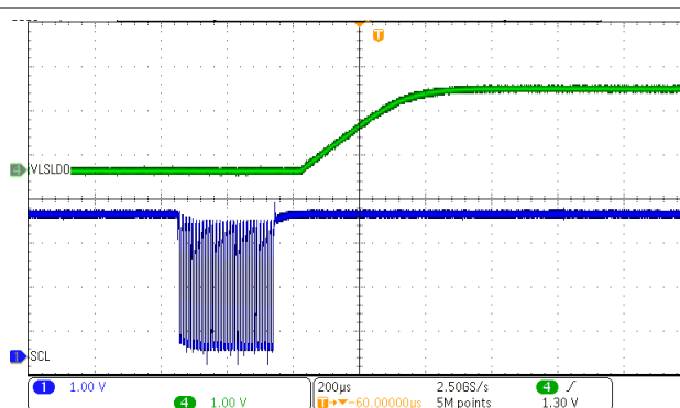
Figure 8-15. LDO Enable Through I2C (EN_LS_LDO)
