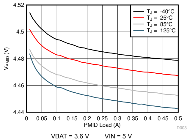
Figure 6-14. PMID Load Regulation vs. Temperature
