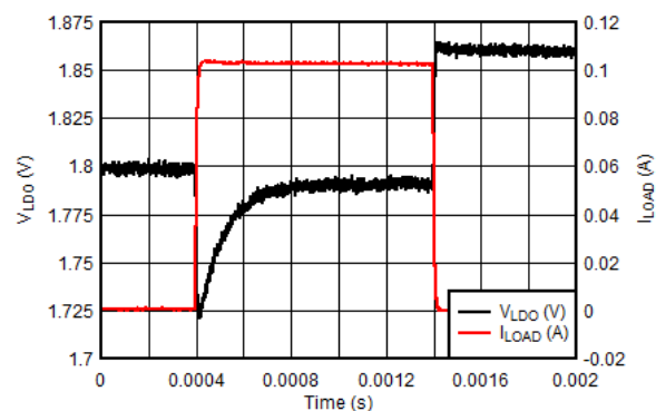
Figure 8-17. LDO Load Transient - VLDO = 1.8V
