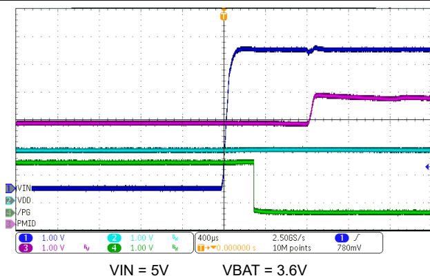
Figure 8-10. \overline{\text{PG}} Power Good Function - IN Supply Insertion
