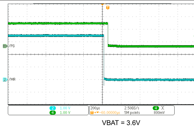
Figure 8-13. \overline{\text{PG}} \overline{\text{MR}} Level Shift Function - \overline{\text{MR}} Falling
