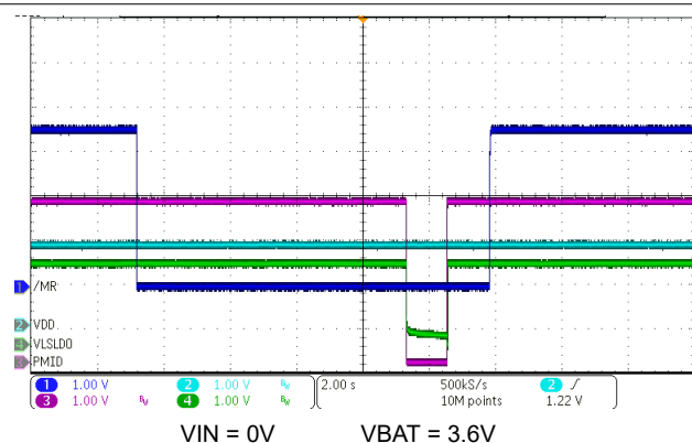
Figure 8-6. HW Reset on \overline{\text{MR}} Long Button Press
