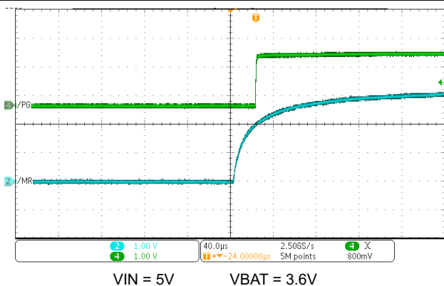
Figure 8-12. \overline{\text{PG}} \overline{\text{MR}} Level Shift Function - \overline{\text{MR}} Rising
