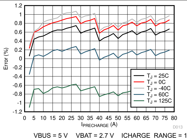
Figure 6-4. Pre-Charge Current Accuracy vs. IPRECHARGE Setting (ICHARGE_RANGE = 1)
