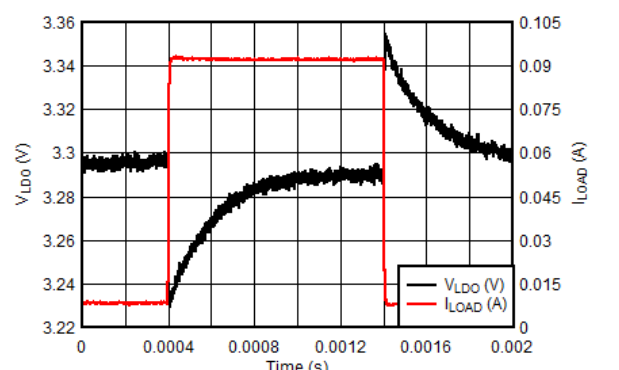
Figure 8-19. LDO Load Transient - VLDO = 3.3V
