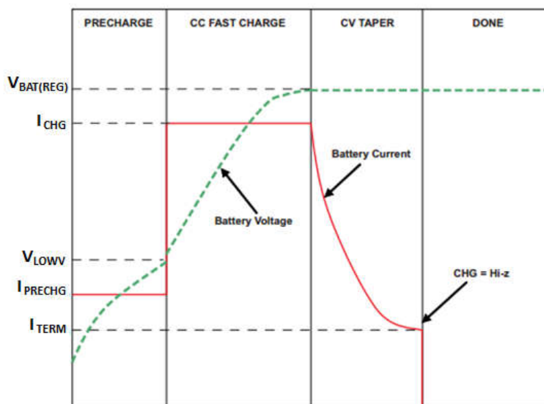
Figure 7-2. BQ21061 Typical Charge Cycle
