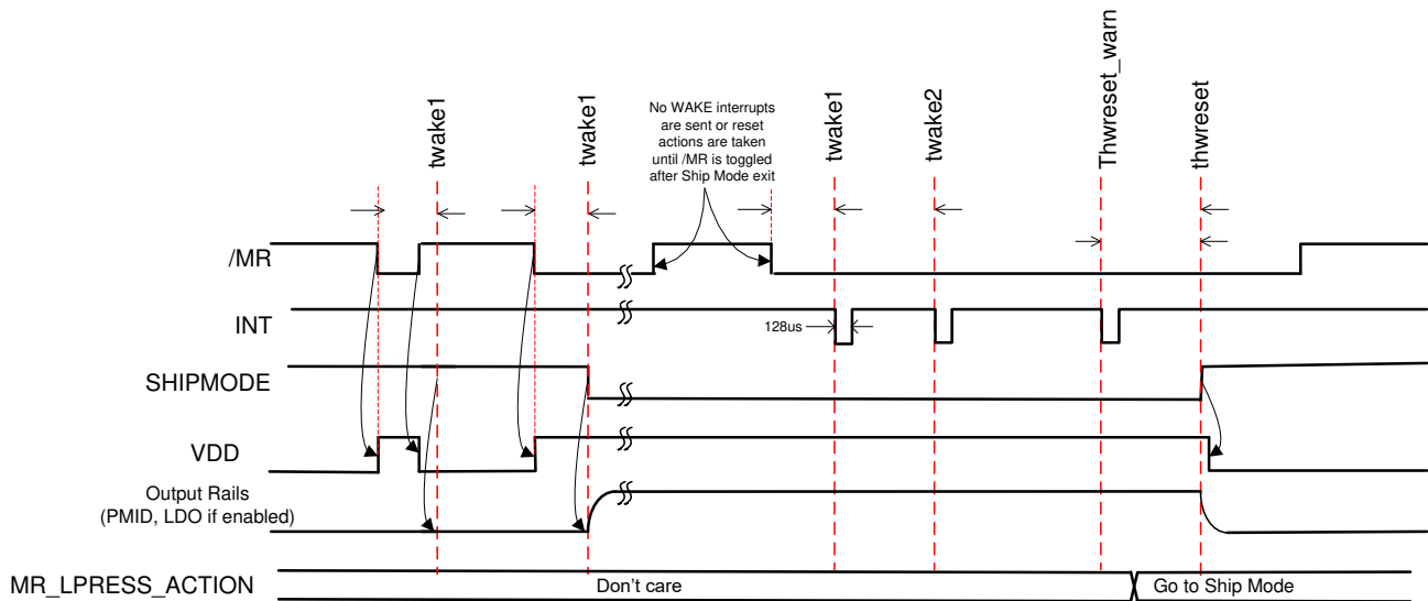
Figure 7-3. MR Wake from Ship Mode ( \text{MR\_LPRESS\_ACTION} = Ship Mode, \text{VIN} not valid)
