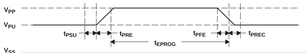
Figure 13. Program Pulse Timing Diagram
