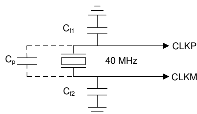
Figure 7-10. Crystal Implementation
