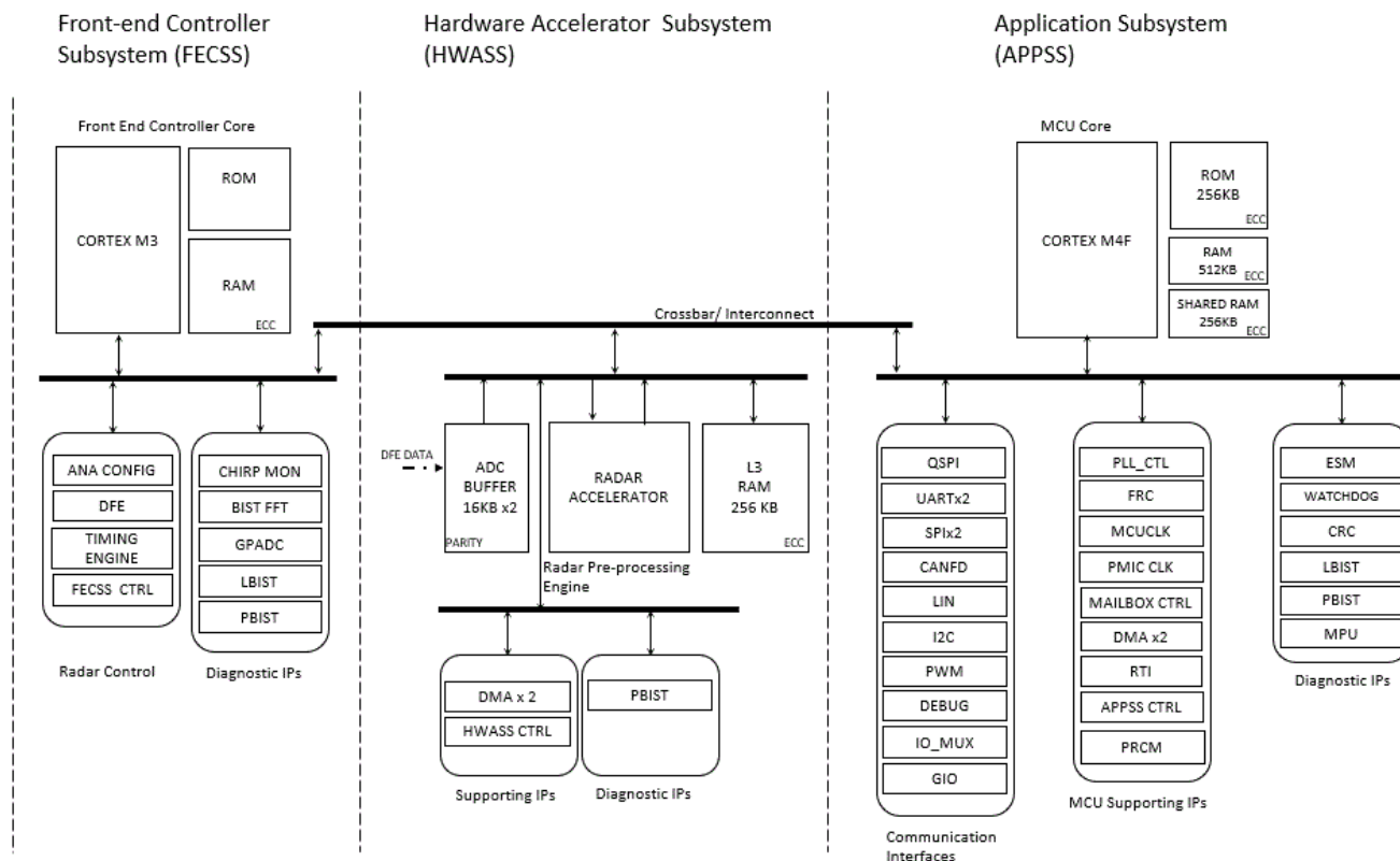
Figure 8-5. Processor Subsystem
