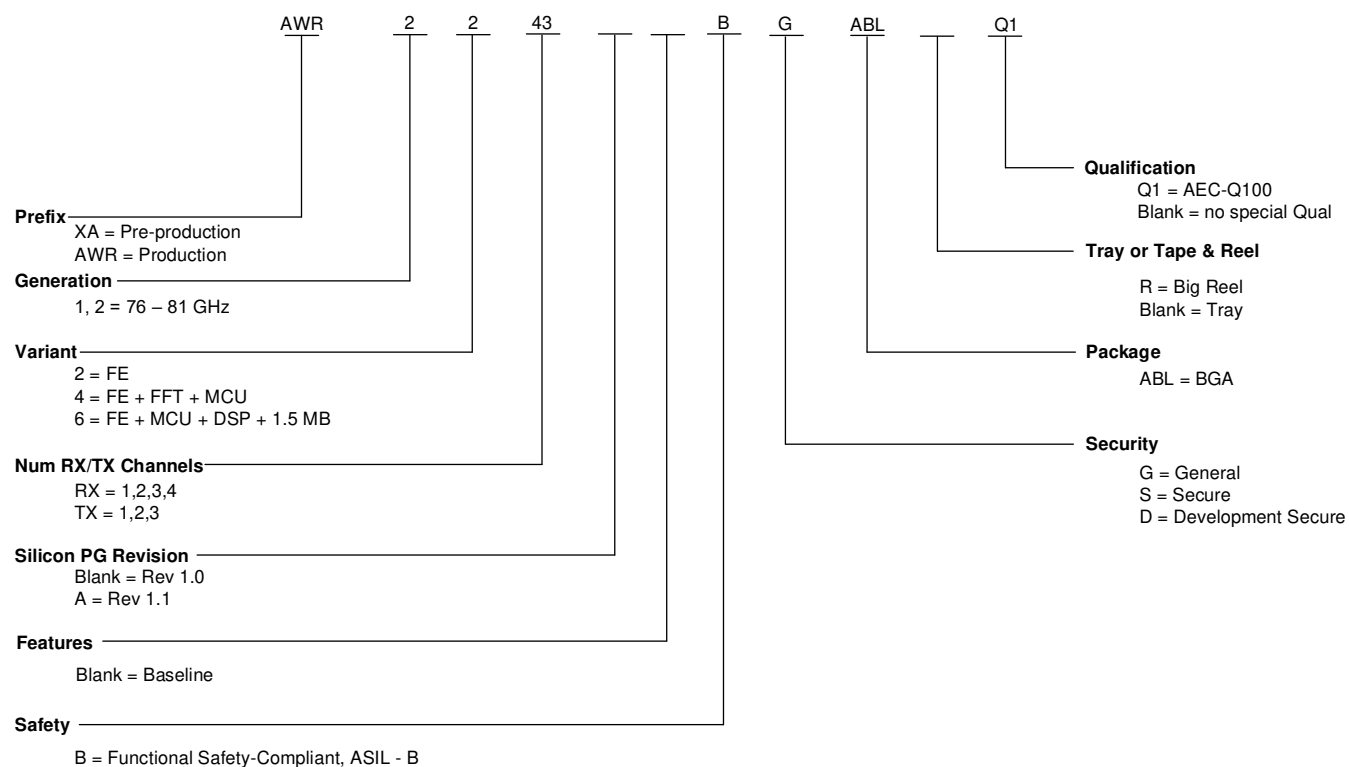
Figure 11-1. Device Nomenclature
