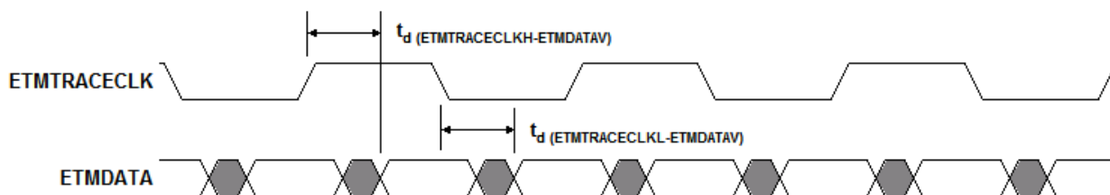
Figure 7-20. ETMDATA Timing
