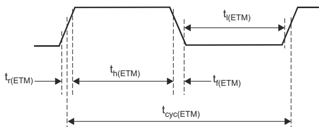
Figure 7-19. ETMTRACECLKOUT Timing
