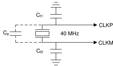
Figure 7-4. Crystal Implementation
