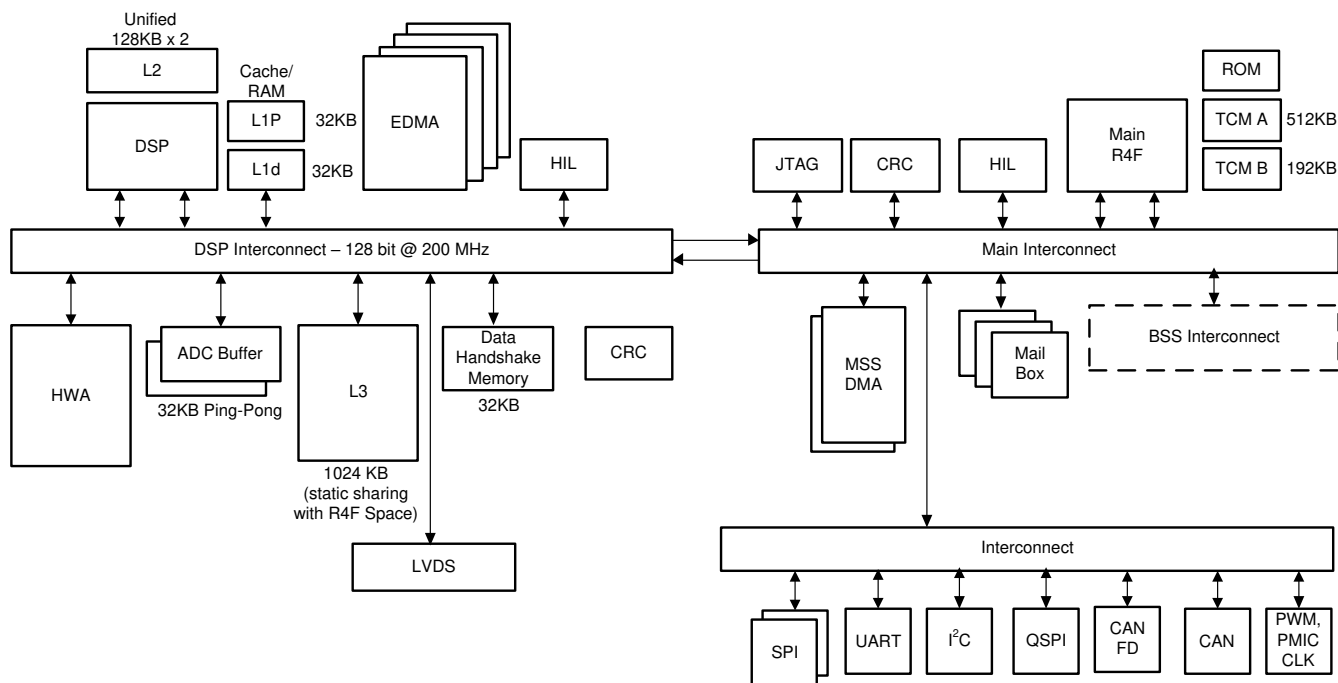
Figure 7-4. Processor Subsystem
