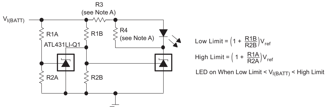
Figure 38. Voltage Monitor
