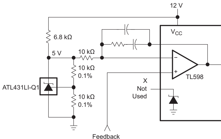
Figure 37. PWM Converter With Reference
