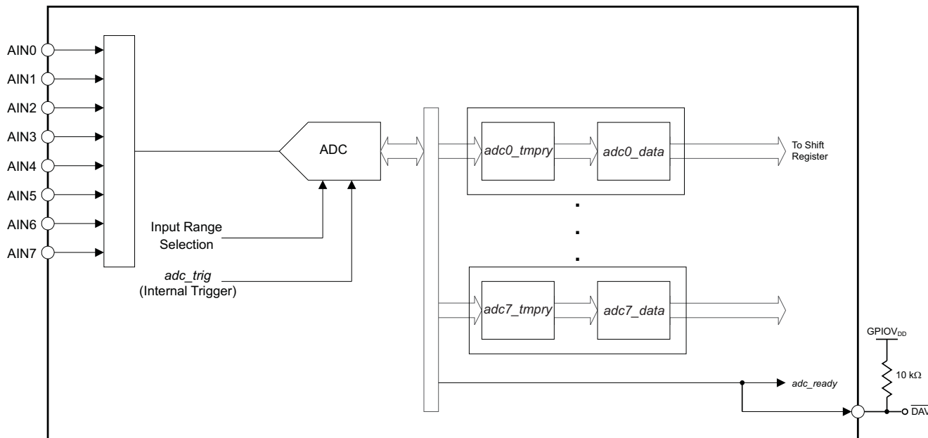
Figure 28. ADC Structure
