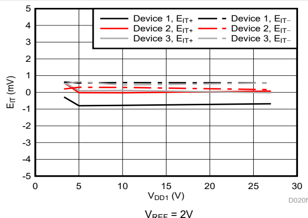
Figure 5-32. Cmp0 Trip Threshold Error vs Supply Voltage
