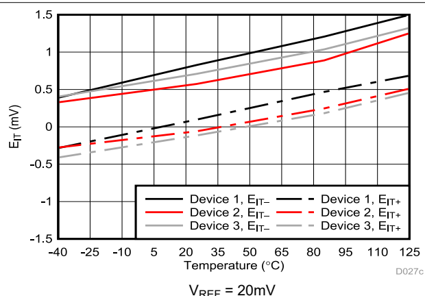
Figure 5-39. Cmp1 Trip Threshold Error vs Temperature
