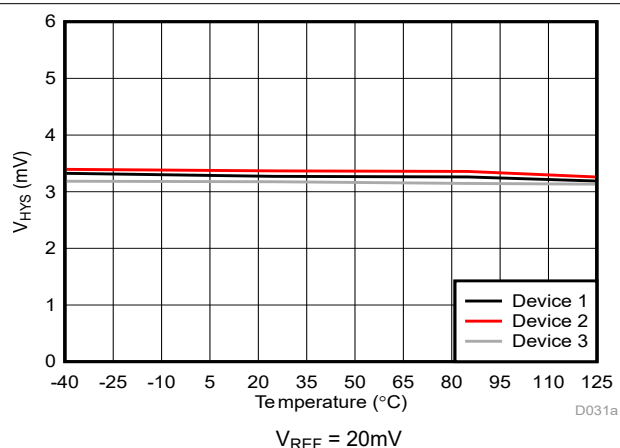
Figure 5-41. Cmp1 Trip Threshold Hysteresis vs Temperature
