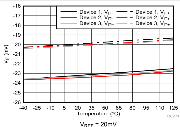
Figure 5-37. Cmp1 Trip Threshold vs Temperature
