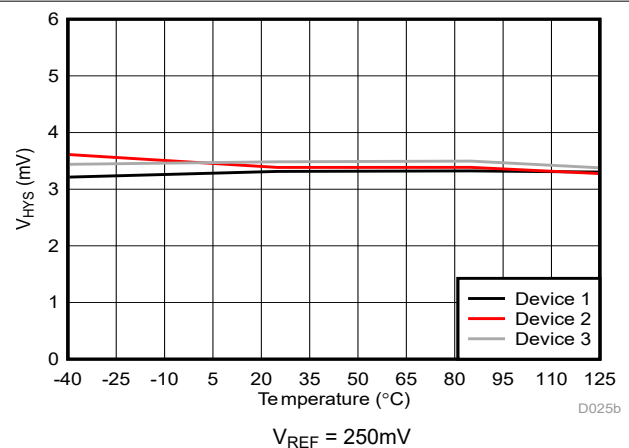
Figure 5-29. Cmp0 Trip Threshold Hysteresis vs Temperature
