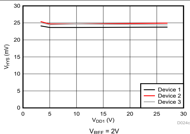
Figure 5-34. Cmp0 Trip Threshold Hysteresis vs Supply Voltage
