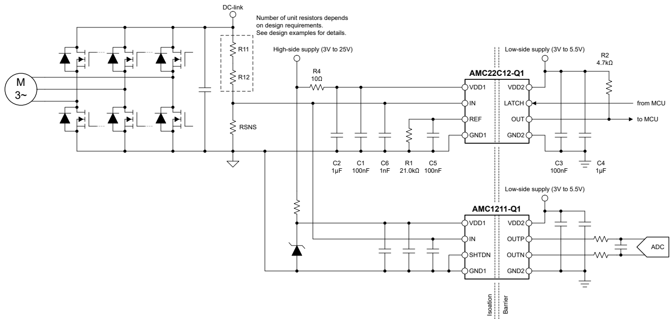
Figure 7-2. Using the AMC22C12-Q1 for Overvoltage Detection
