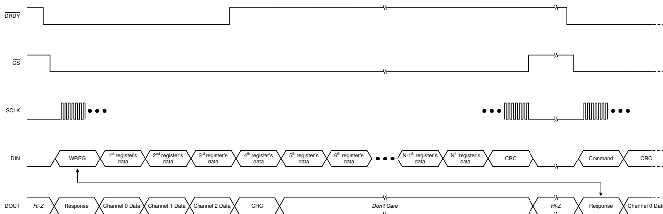
Figure 8-29. Writing Registers
