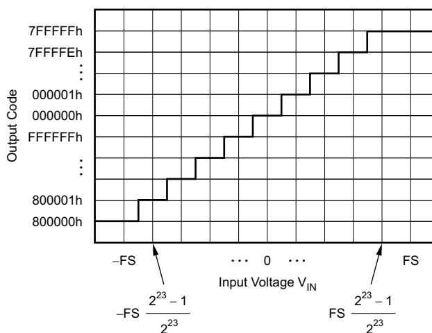
Figure 8-25. Code Transition Diagram
