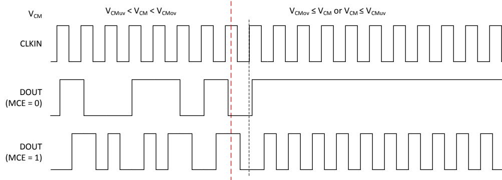
Figure 44. Fail-Safe Output of the AMC1035-Q1
