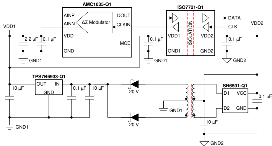
Figure 49. Galvanic Isolation of the AMC1035-Q1
