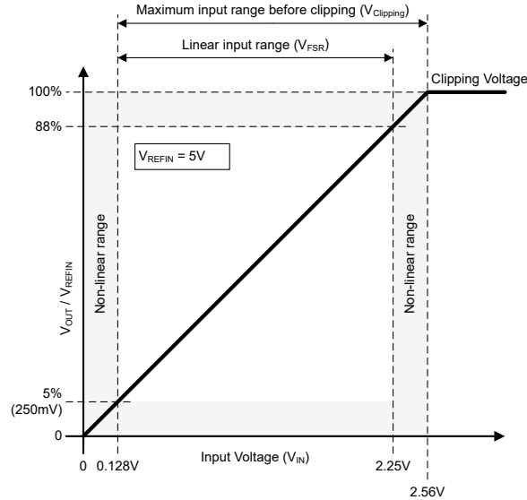
Figure 7-2. Input to Output Transfer Curve of the AMC0x11R
