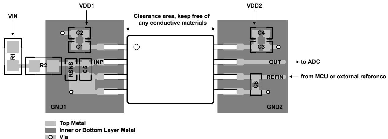
Figure 8-6. Recommended Layout of the AMC0x11R
