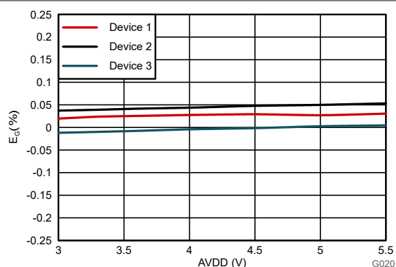
Figure 6-14. Gain Error vs High-Side Supply Voltage
