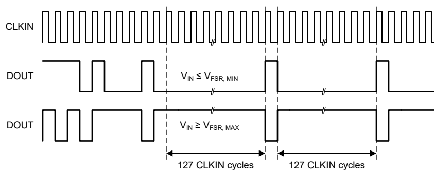
Figure 7-6. Full-Scale Output of the AMC0x06M25
