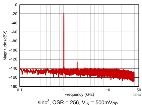
Figure 6-38. Frequency Spectrum With 1kHz Input Signal
