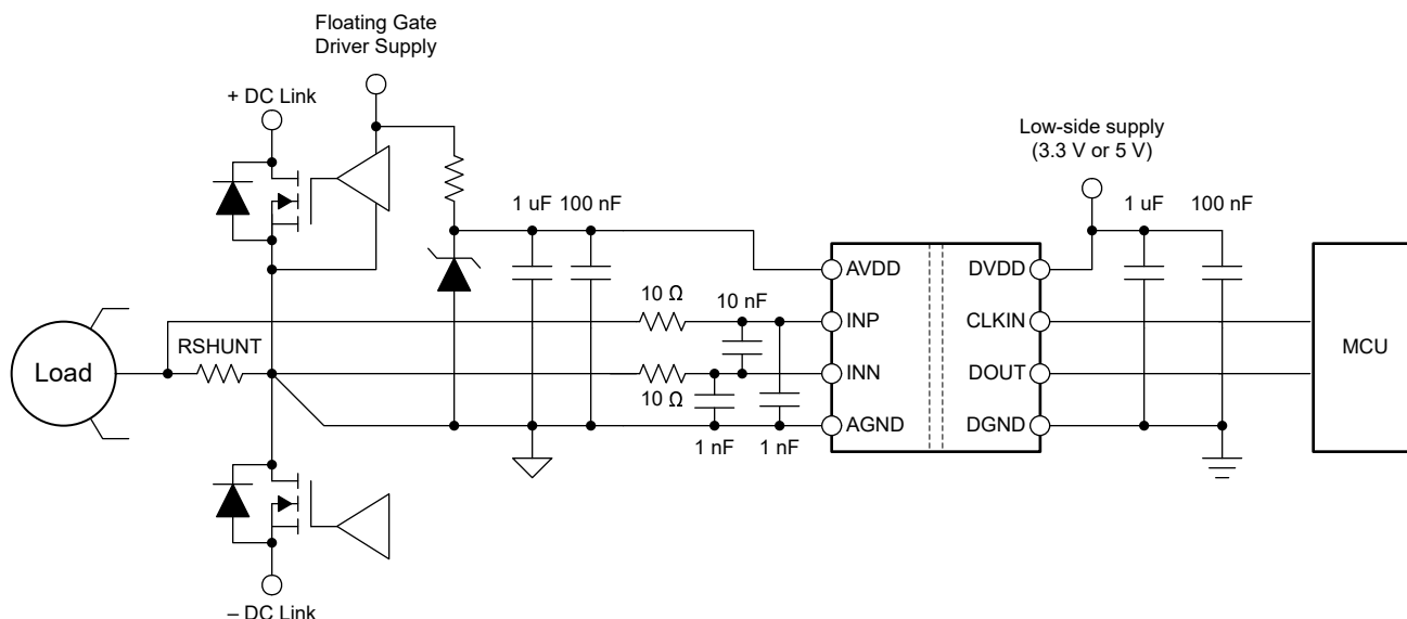
Figure 8-1. Using the AMC0x06M25 for Current Sensing in a Typical Application
