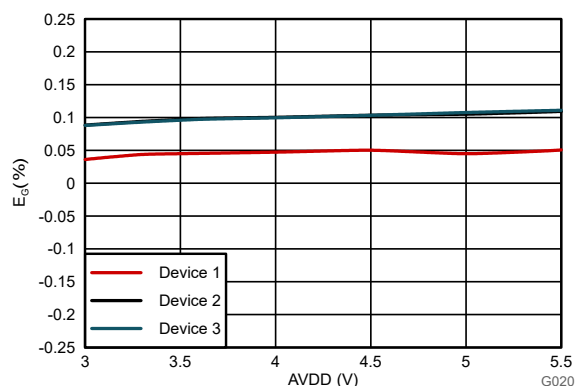
Figure 5-10. Gain Error vs High-Side Supply Voltage
