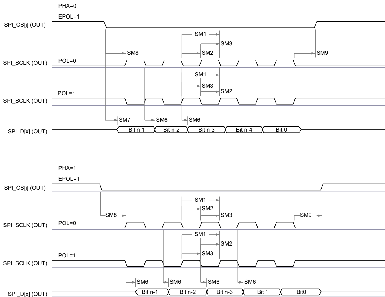
Figure 6-65. SPI Controller Mode Transmit Timing
