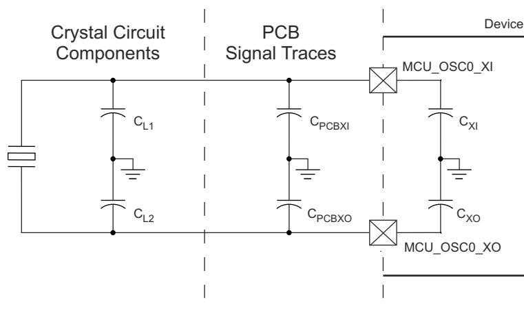
Figure 6-18. Load Capacitance
