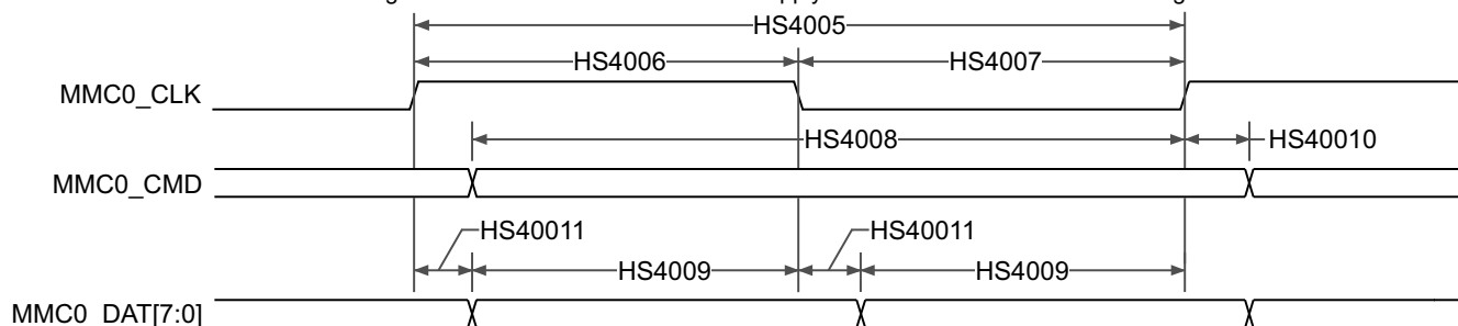
Figure 6-76. eMMC in – HS400 Mode – Transmitter Mode
