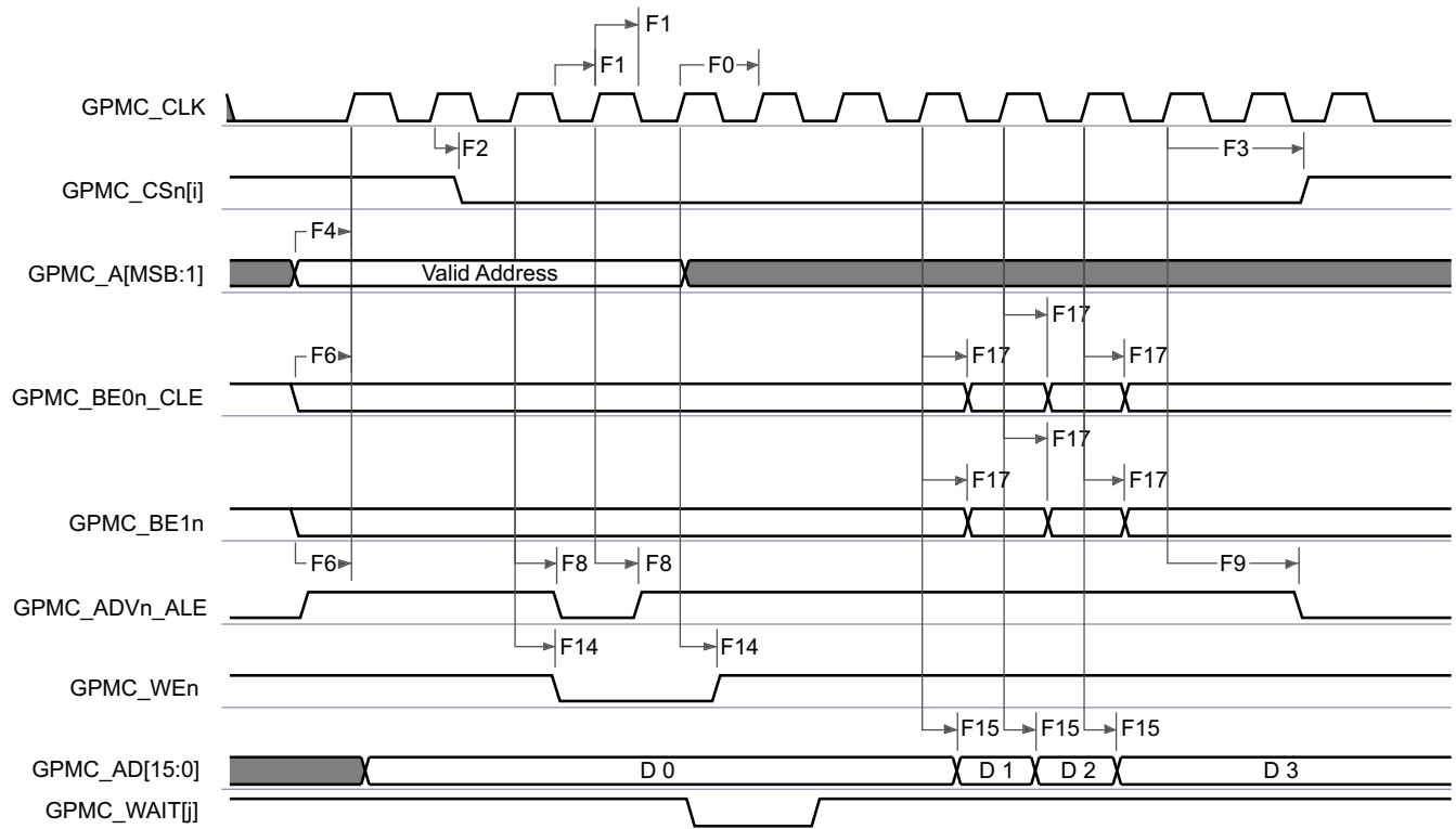
Figure 6-48. GPMC and NOR Flash — Synchronous Burst Read — 4x16-bit (GPMCCLKDIVIDER = 0)
