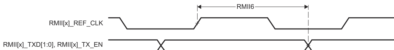
Figure 6-30. RMII[x]_TXD[1:0], and RMII[x]_TX_EN Switching Characteristics – RMII Mode
