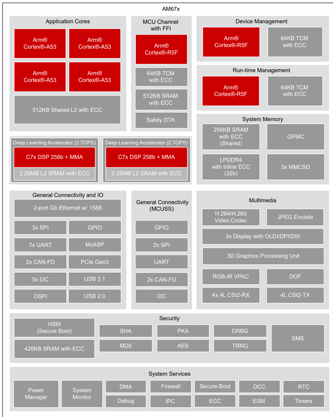
Figure 3-1. Functional Block Diagram
