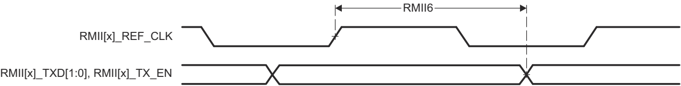
Figure 6-25. RMII[x]_TXD[1:0], and RMII[x]_TX_EN Switching Characteristics – RMII Mode
