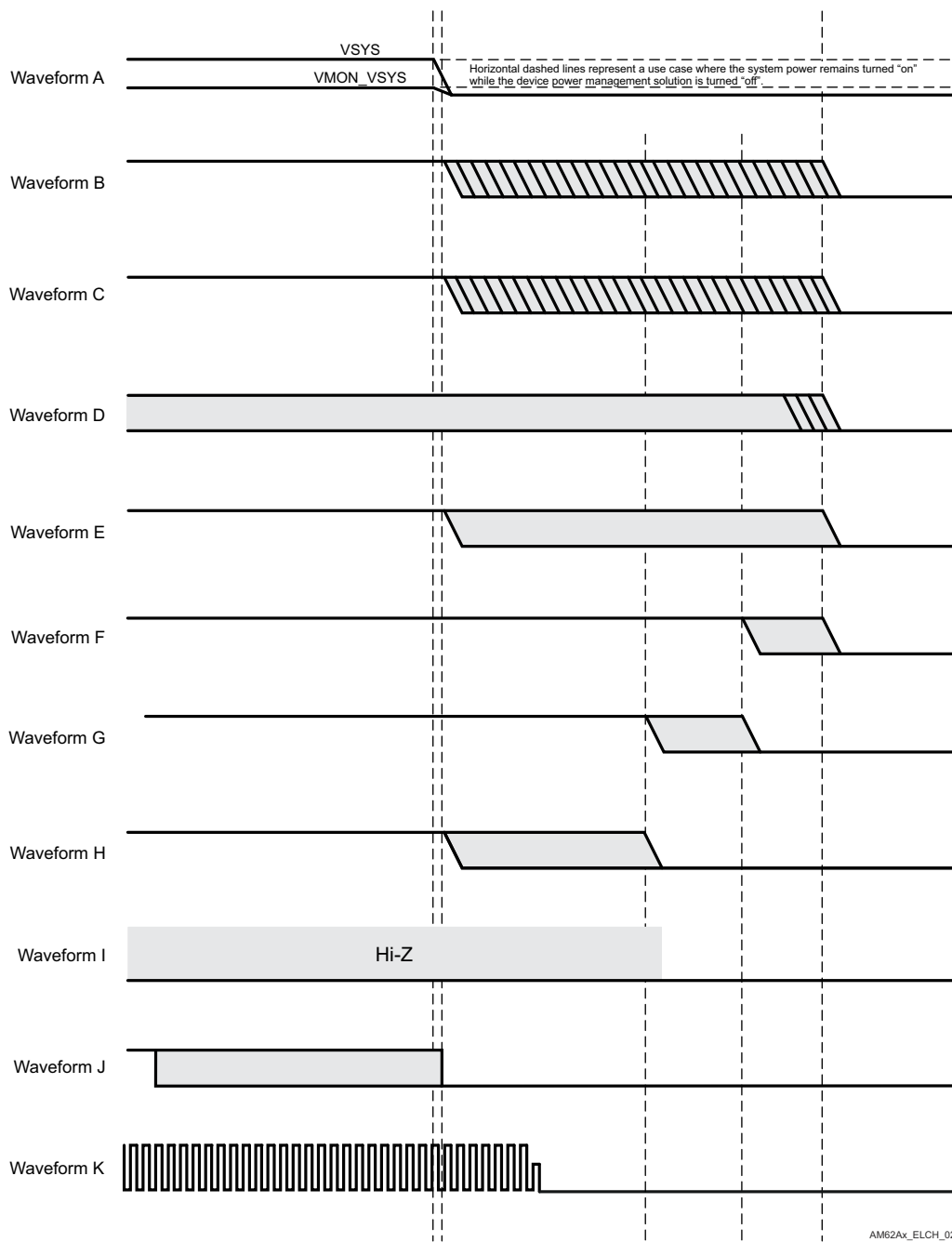
Figure 6-6. Power-Down Sequencing
