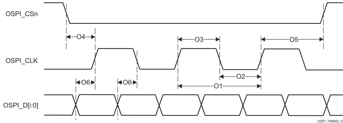
Figure 6-97. OSPI0 Switching Characteristics – PHY DDR
