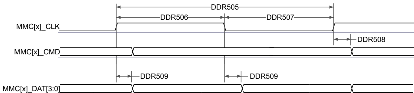
Figure 6-86. MMC1/MMC2 – UHS-I DDR50 – Transmit Mode
