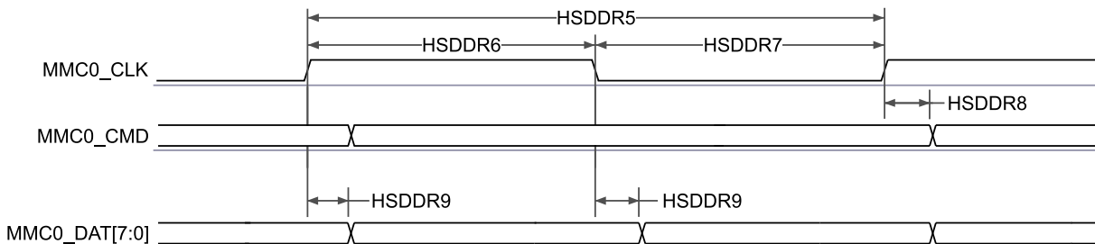
Figure 6-76. MMC0 – High Speed DDR Mode – Transmit Mode
