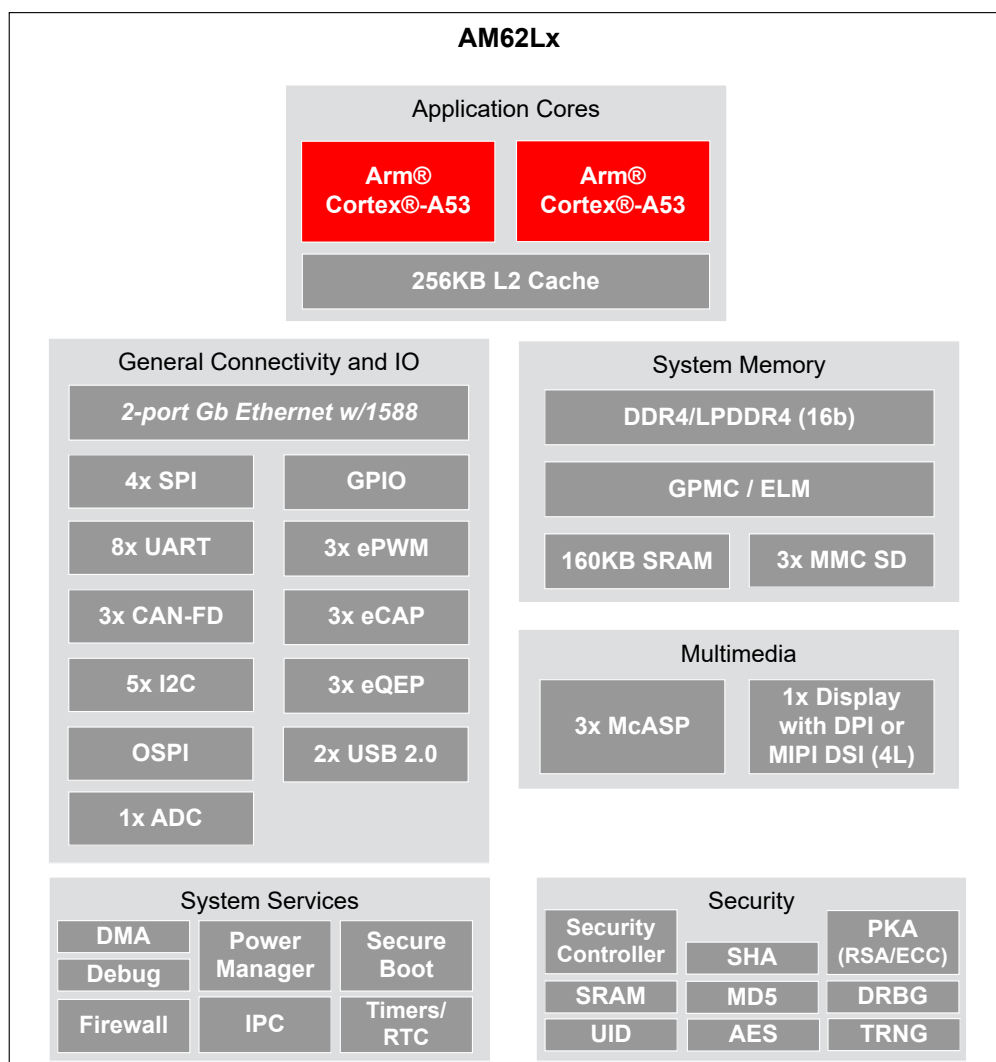
Figure 3-1. Functional Block Diagram
