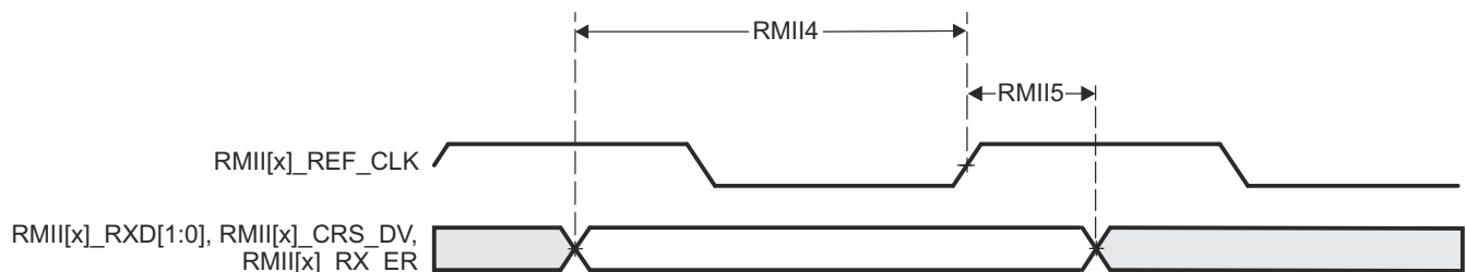
Figure 6-32. CPSW3G RMII[x]_RXD[1:0], RMII[x]_CRS_DV, RMII[x]_RX_ER Timing Requirements – RMII Mode
