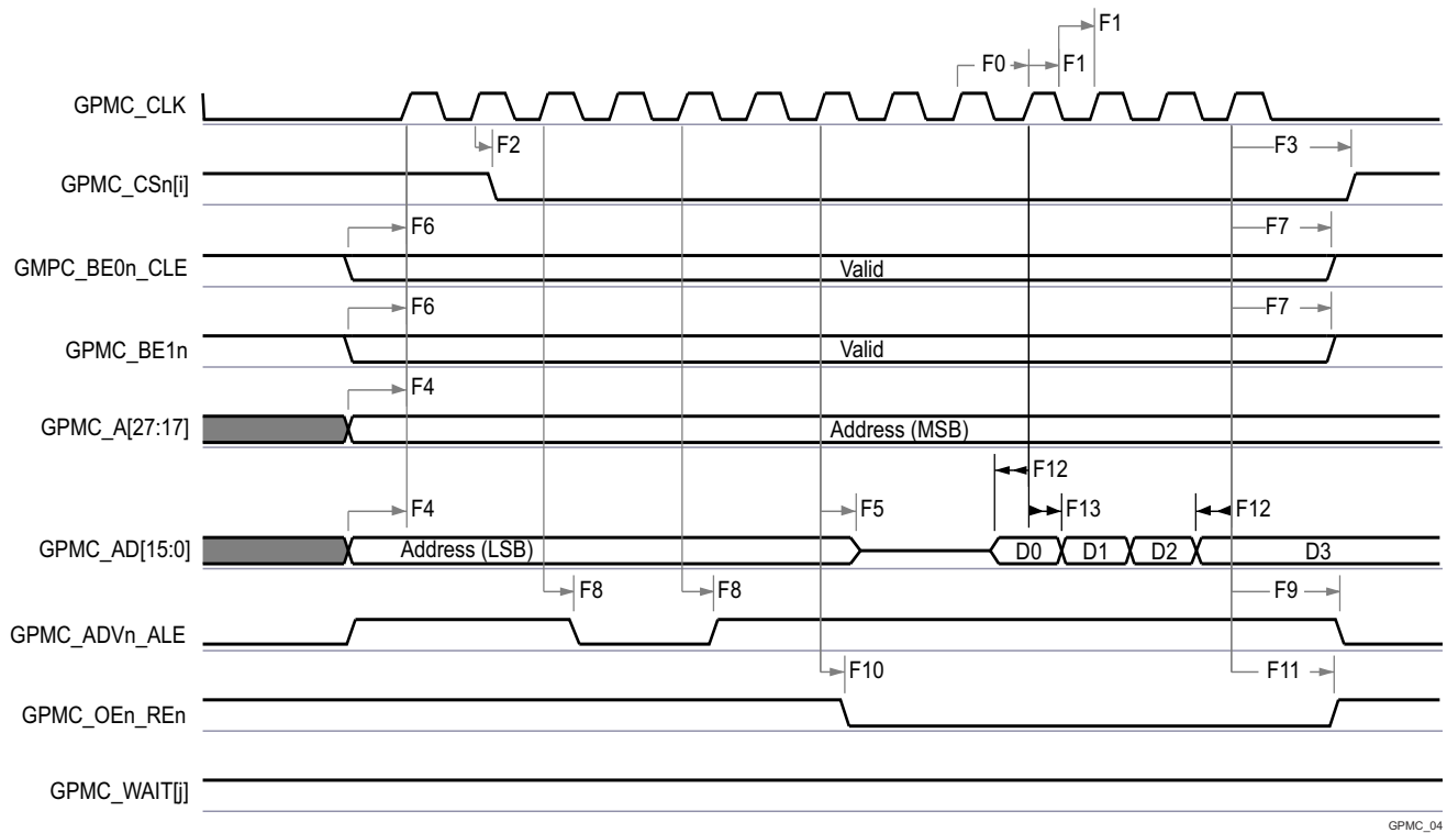
Figure 6-44. GPMC and NOR Flash—Synchronous Burst Write (GPMCFCLKDIVIDER = 0)
