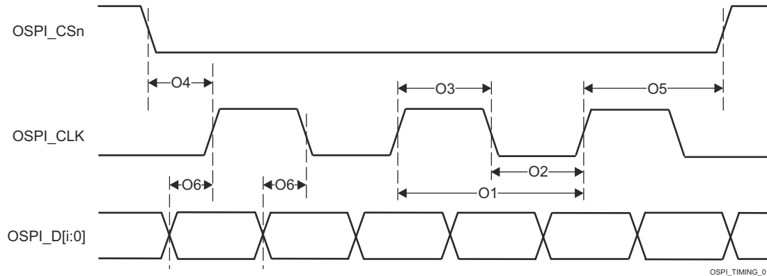
Figure 6-100. OSPI0 Switching Characteristics – PHY DDR
