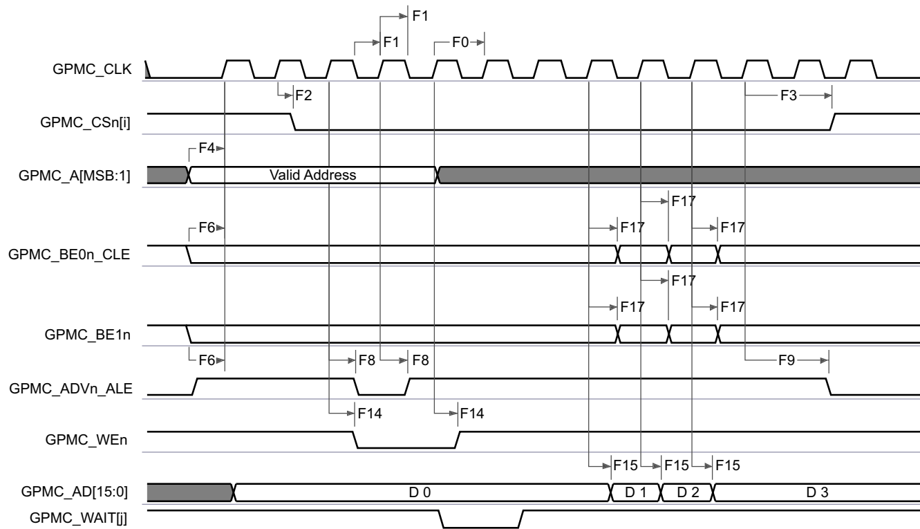
Figure 6-43. GPMC and NOR Flash — Synchronous Burst Read — 4x16-bit (GPMCFCLKDIVIDER = 0)
