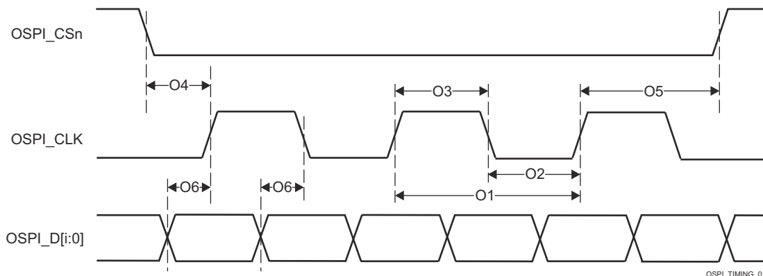
Figure 6-94. OSPI0 Switching Characteristics – PHY DDR Data Training
