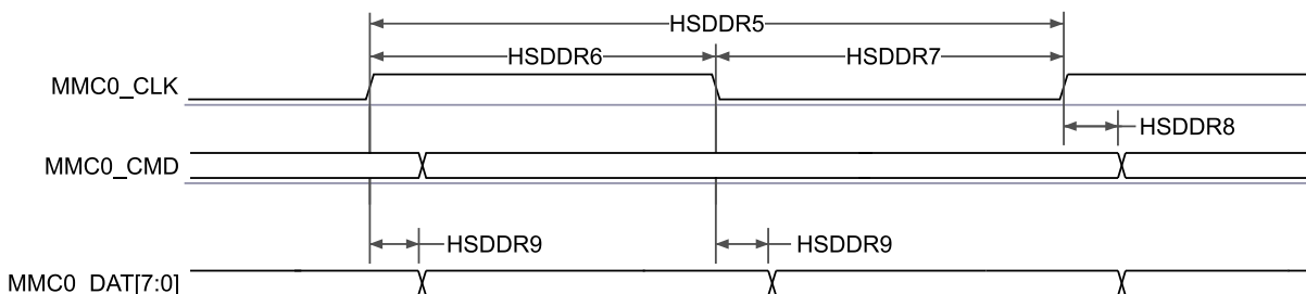
Figure 6-68. MMC0 – High Speed DDR Mode – Transmit Mode
