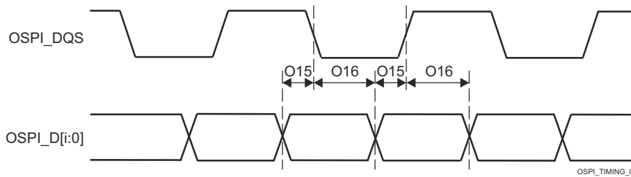
Figure 6-99. OSPI0 Timing Requirements – PHY DDR with External Board Loopback or DQS
