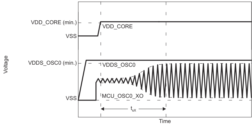
Figure 6-17. MCU_OSC0 Start-up Time
