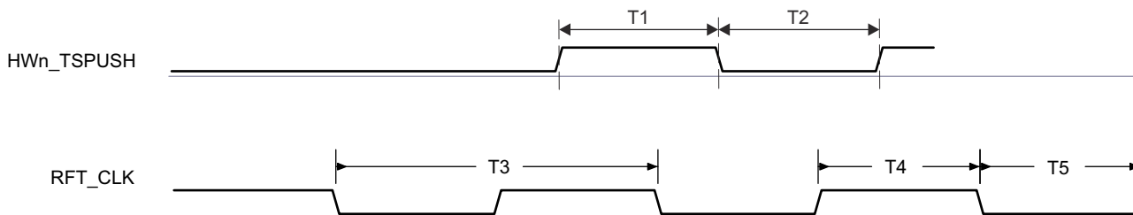
Figure 6-30. CPTS Timing Requirements
