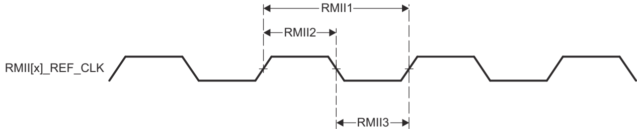
Figure 6-25. CPSW3G RMII[x]_REF_CLK Timing Requirements – RMII Mode
