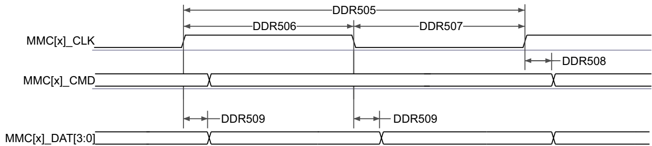
Figure 6-79. MMC0 – UHS-I DDR50 – Transmit Mode
