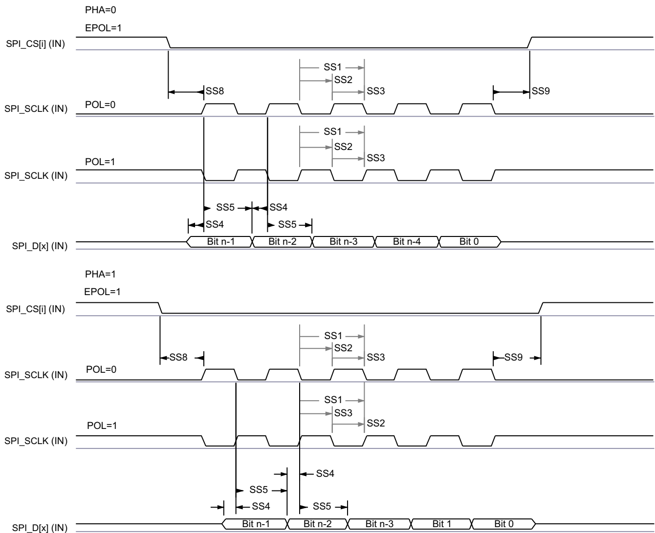
Figure 6-61. SPI Peripheral Mode Receive Timing
