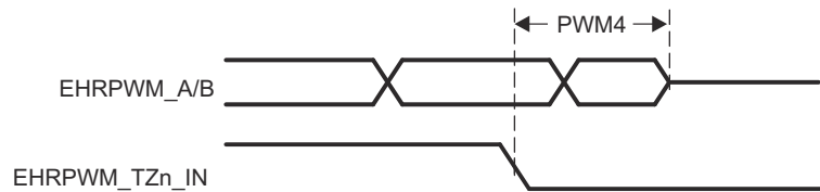
Figure 6-40. EHRPWM_TZn_IN to EHRPWM_A/B Hi-Z Switching Characteristics
