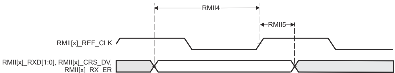
Figure 6-26. CPSW3G RMII[x]_RXD[1:0], RMII[x]_CRS_DV, RMII[x]_RX_ER Timing Requirements – RMII Mode
