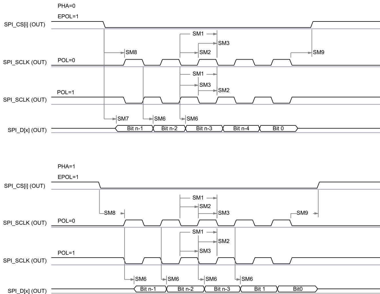
Figure 6-60. SPI Controller Mode Transmit Timing
